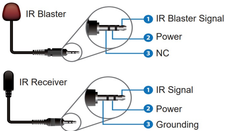
Connection diagram of using IR cables.
