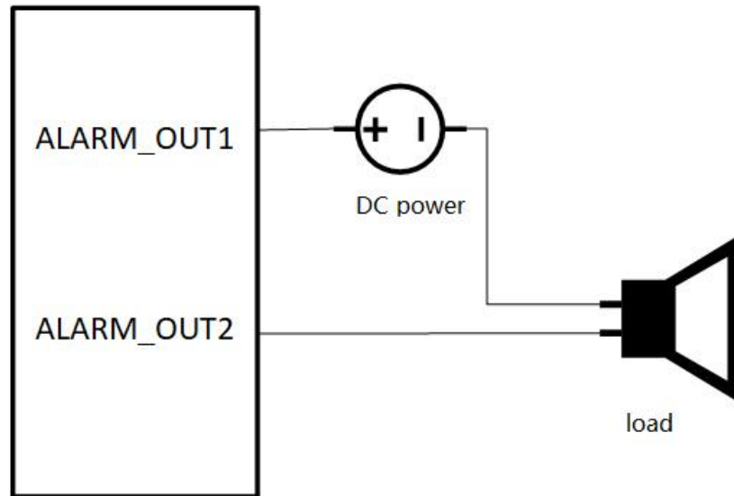
Figure 2.3 Wiring Method of Alarm Output
