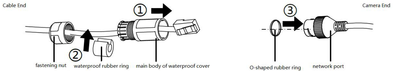
Figure 2.7 Network Cable Installation
