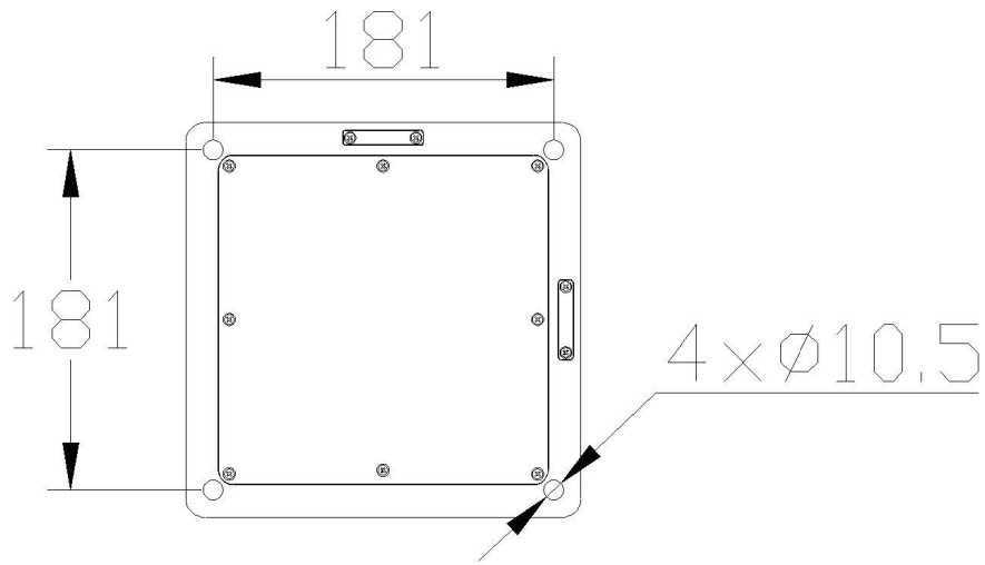
Figure 2.8 PT Installation Dimensions
