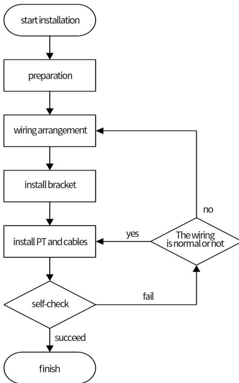
Figure 2.4 Mounting Process
