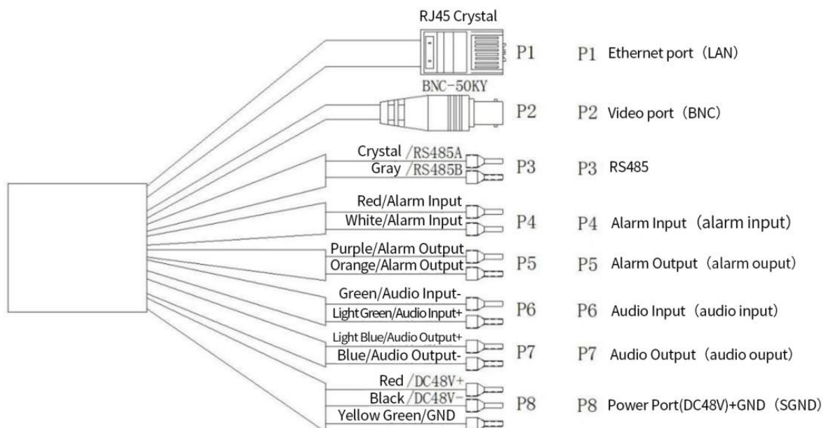
Figure 2.2 Cable Introduction
