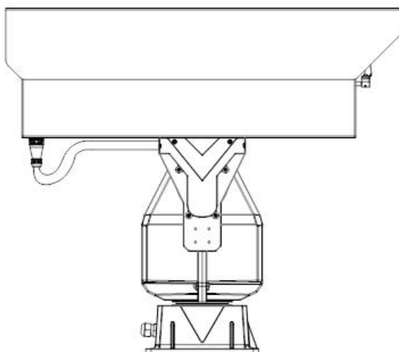
Figure 2.7 Connect Cables of the Protective Cover
