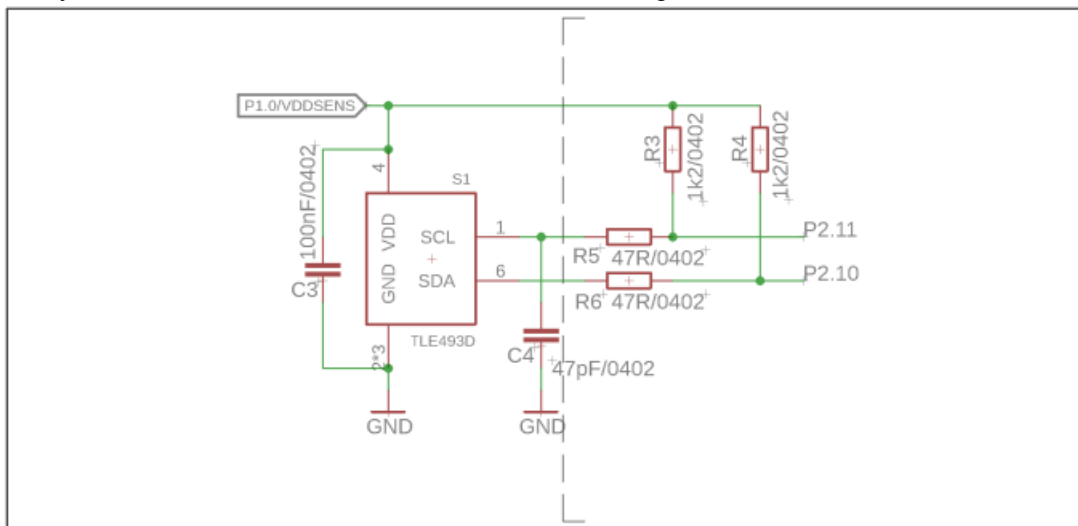
Figure 9 EvalBoard schematic: 3D magnetic sensor
