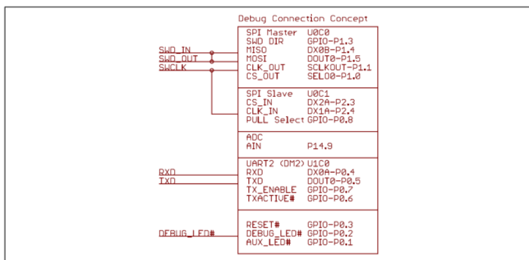
Figure 13 Sketch of the debug connection
