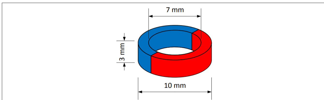
Figure 5 Magnet used in the out of shaft extension
