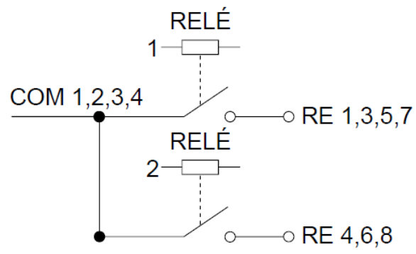
a) Relay
