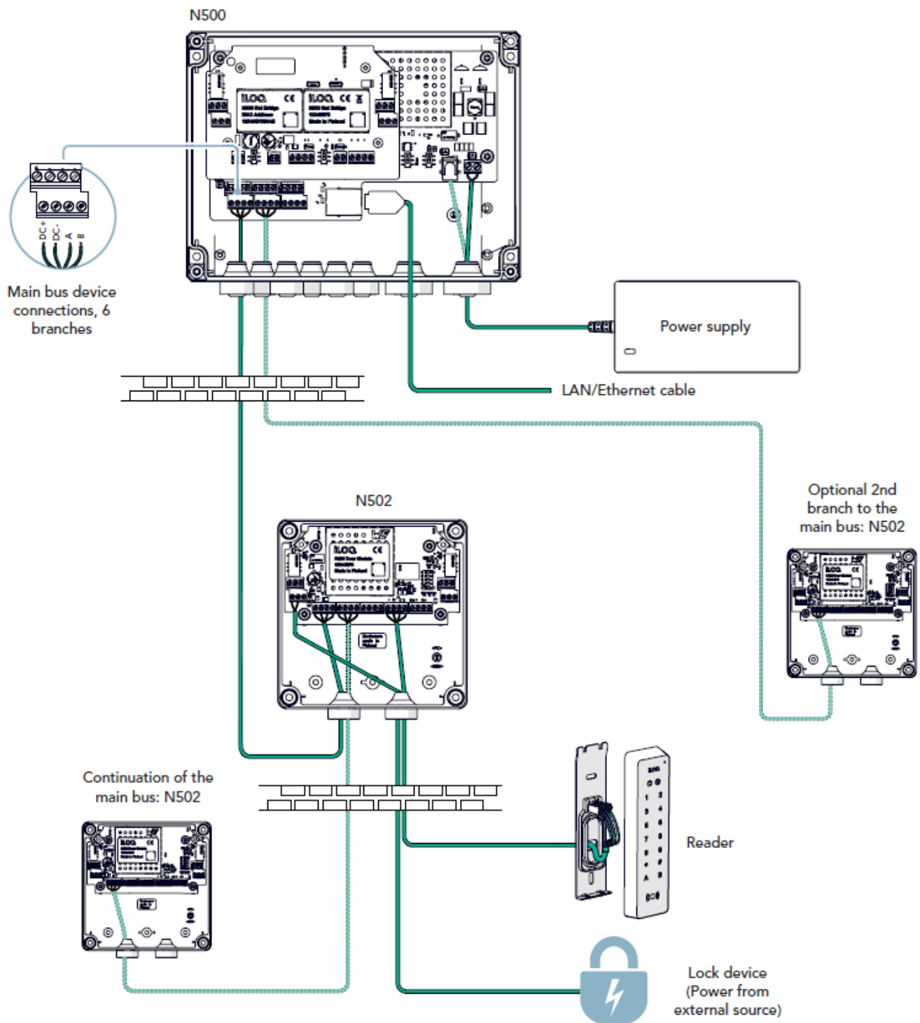
Example of wiring iLOQ N500-N507
