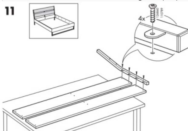
IKEA TRYSIL Bed Frame - Fig 20 (11)
