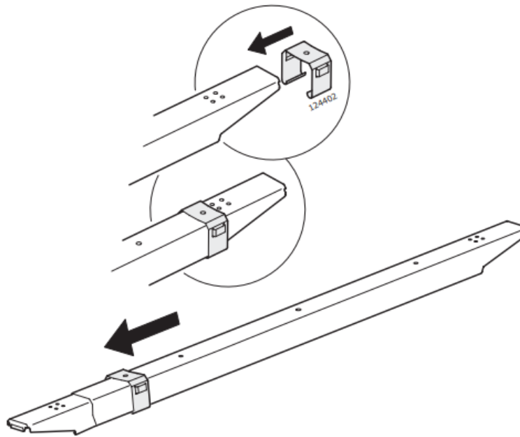
IKEA TRYSIL Bed Frame - Fig 20 (18)
