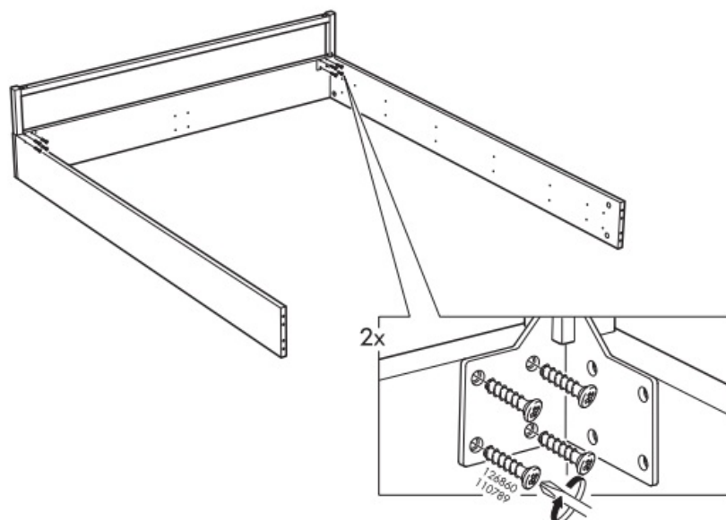
IKEA TRYSIL Bed Frame - Fig 20 (10)
