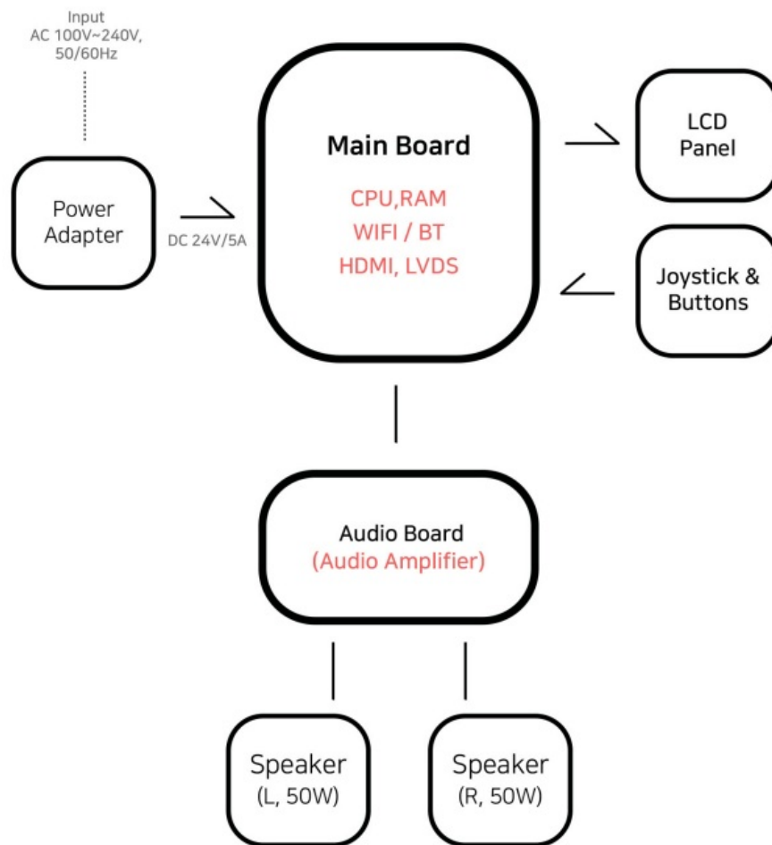
iiRcade Mainboard configuration
