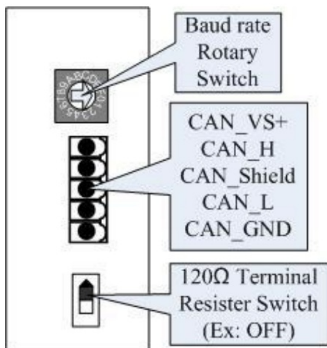
Figure 2-1 CAN-2053C layout of LED, connect, and switch
