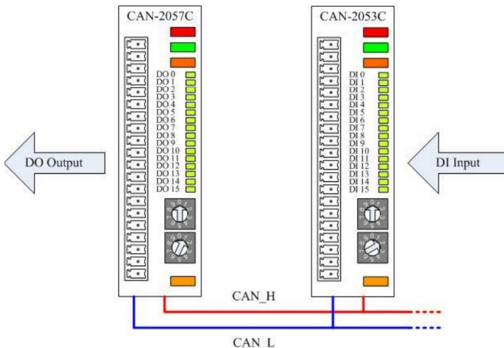
Figure 2-5 I/O pair-connection wire connect
