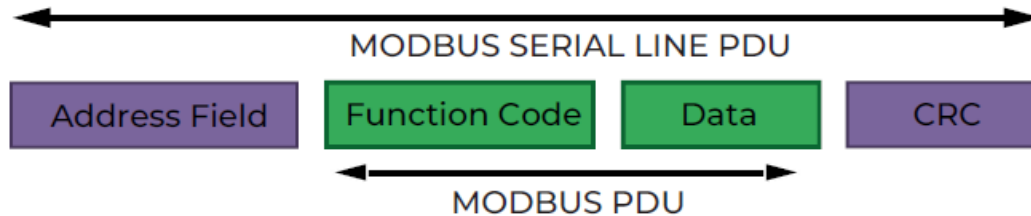
Fig.2 : MODBUS Architecture for Serial Communication
