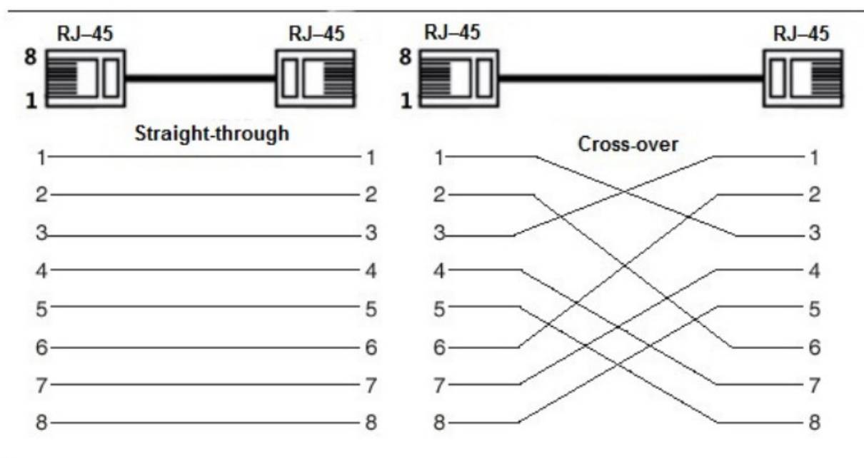
Figure 4-3 Pin description
