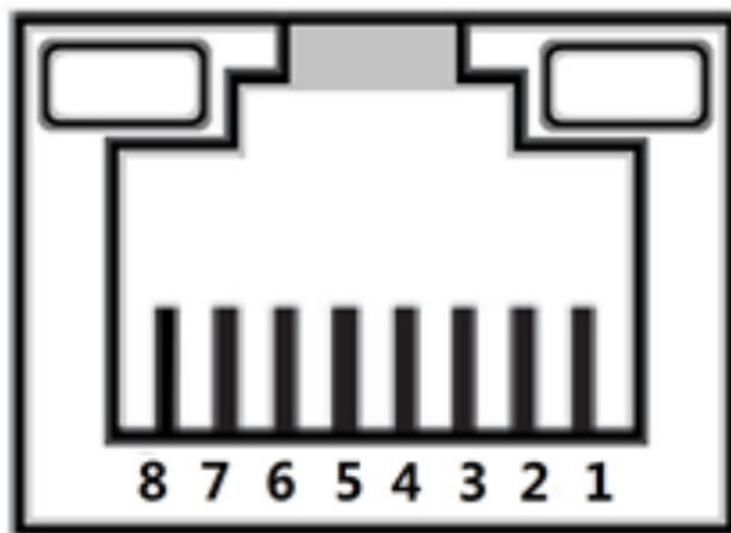
Figure 4-3 Pin description
