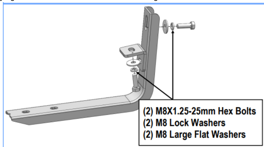
(Fig 4) Passenger Front Mounting Bracket Installation
