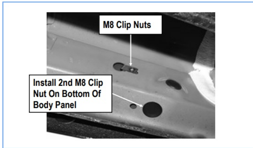
(Fig 3) Slide M8 Clip Nut Into Large Hole And Over Small Hole
