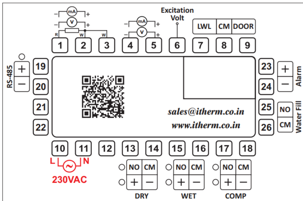
Front panel layout
