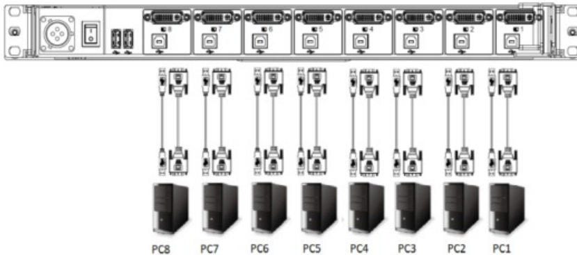
Figure 3. Computer/Server Installation
