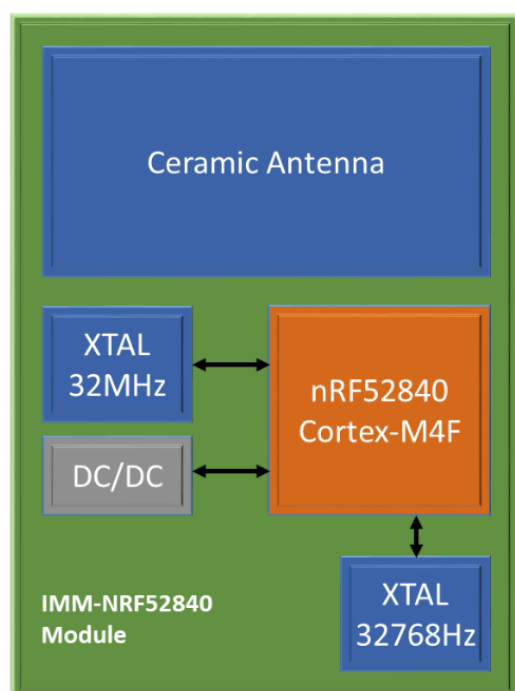
Figure 1: Module internal diagram
