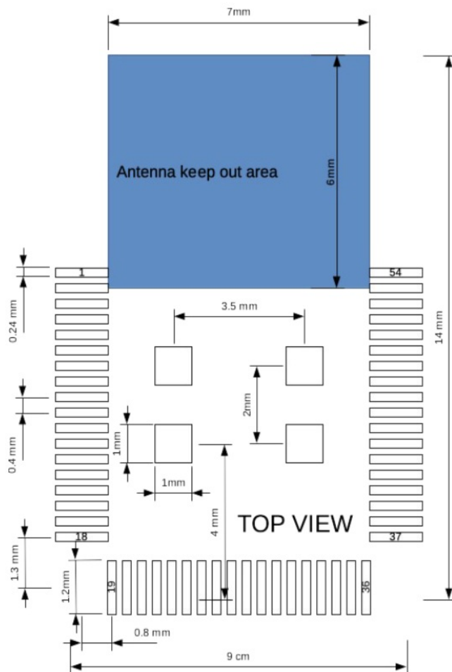
Figure 4: SMD footprint top view
