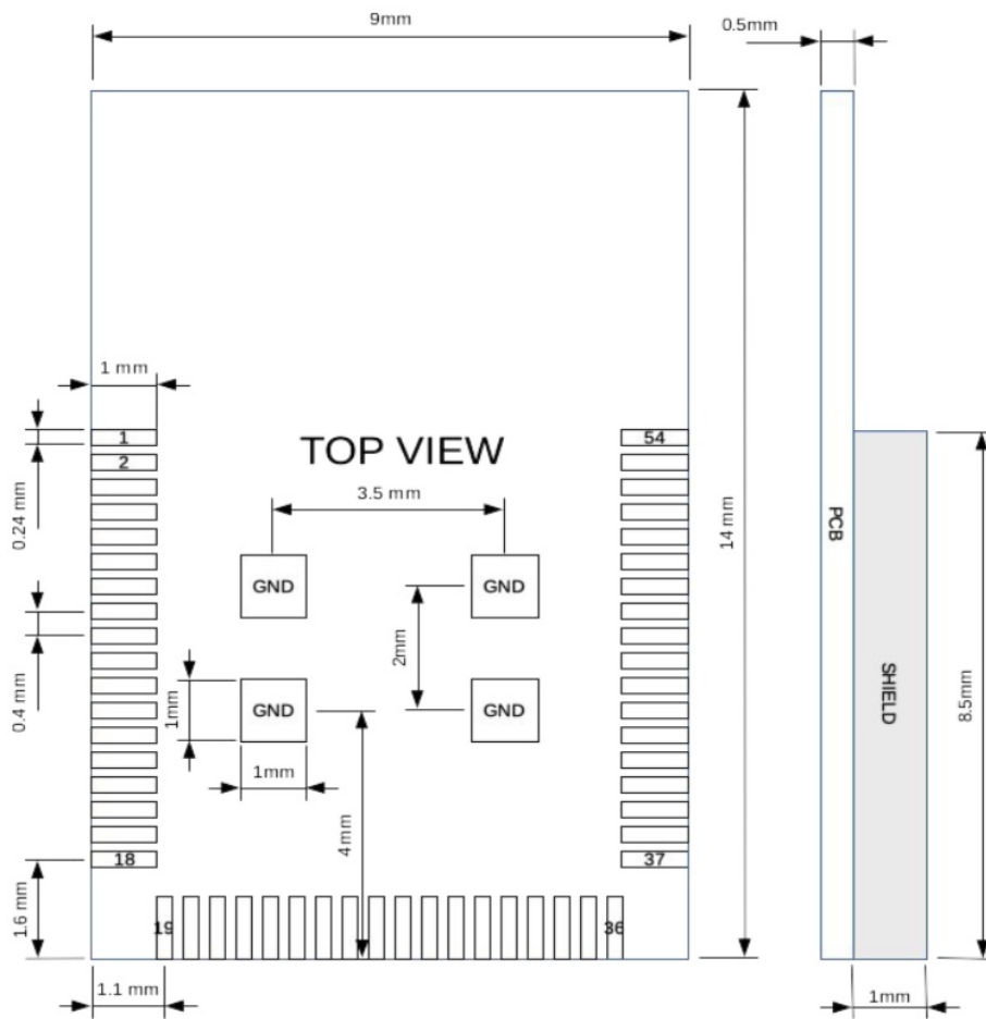
Figure 2: Dimensions top view
