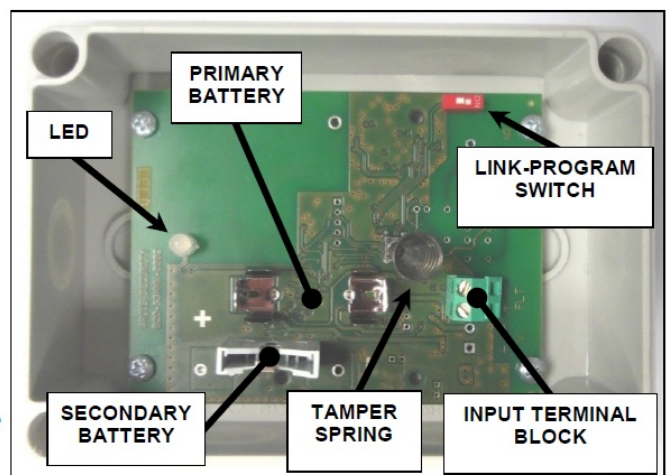
Picture 2 - The PCB of the device
