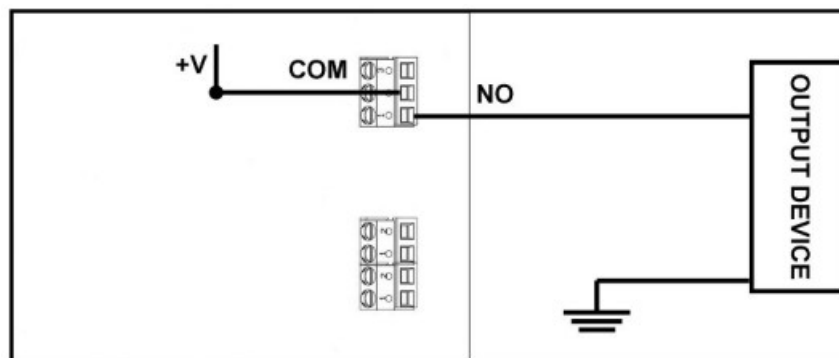
Picture 7 – Wiring example for relay switch output
