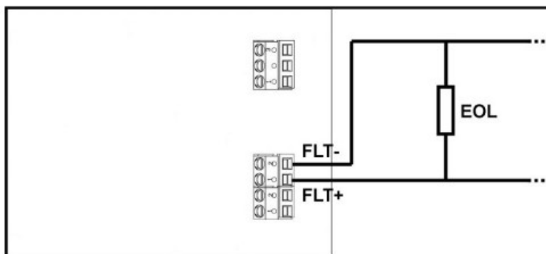
Picture 8 – Wiring example for the FLT port
