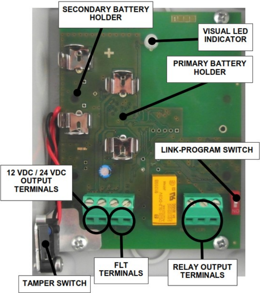
Picture 2 – PCB detail
