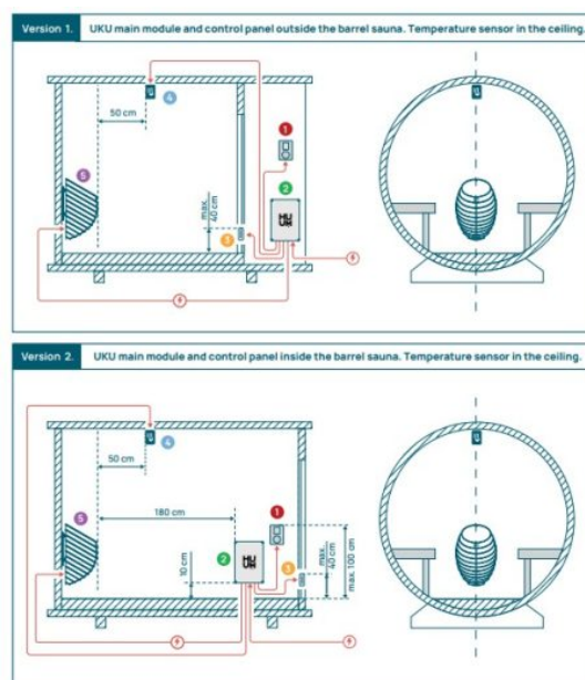
Figure 4. HUUM UKU installation in barrel saunas.
