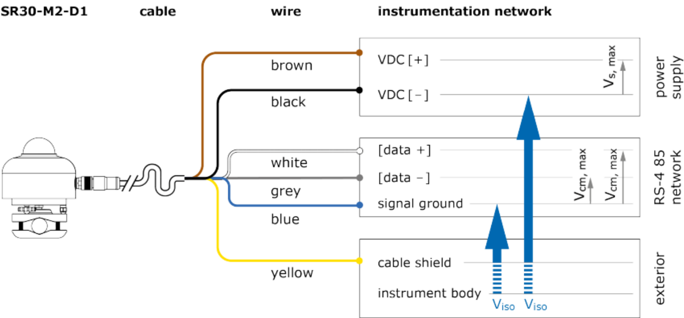
Figure 5.4.1 Electrical connections of SR30-M2-D1.
