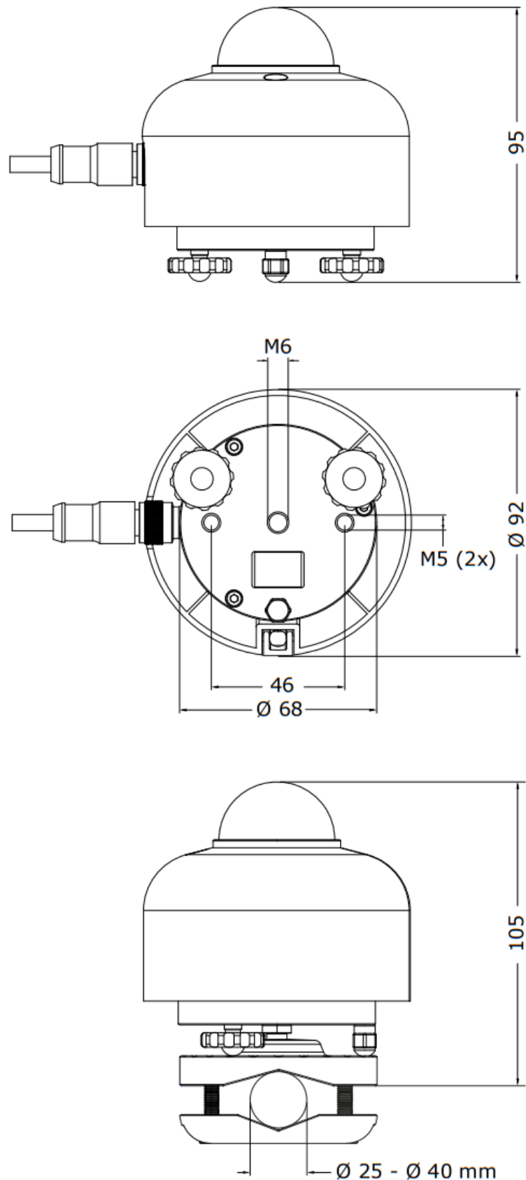
Figure 3.2.1 Dimensions of SR30-M2-D1 in x 10 -3 m. Mounts are optional.
