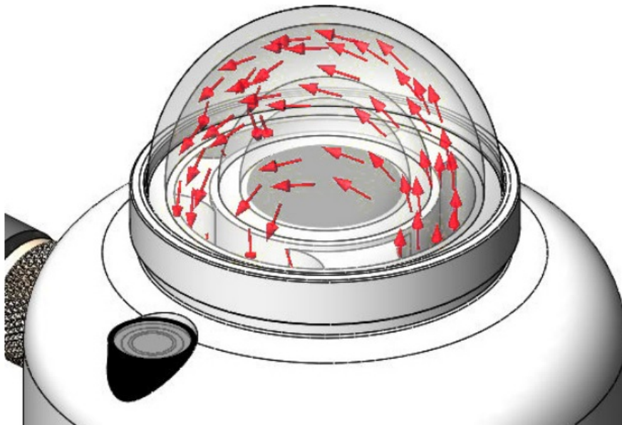
Figure 2.1.1 Heating: how it's done: recirculating ventilation and heating between the inner- and outer dome forming a closed circuit with the body is much more power efficient than traditional ventilation systems.
