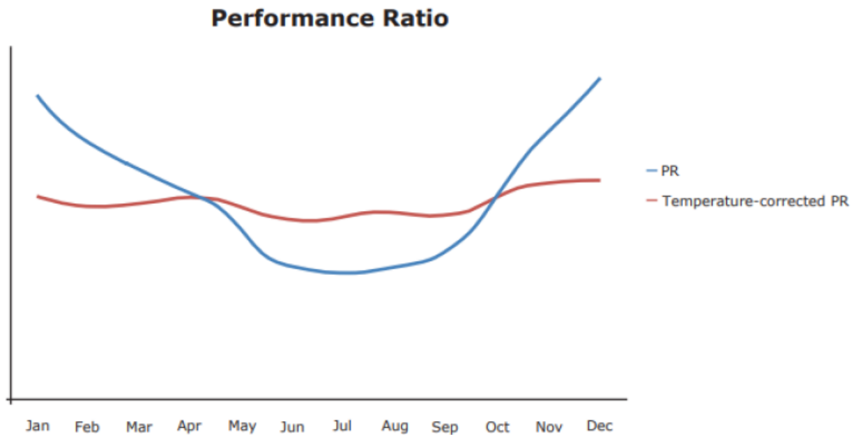
Figure 2.3.1. Performance ratio (PR) with and without temperature correction. This schematic graph is for a PV system located in the northern hemisphere. Temperature measurements with PVMT01 can be used for temperature correction.
