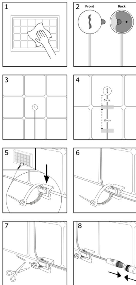
Figure 4.1.1 PVMT01 installation instructions.
