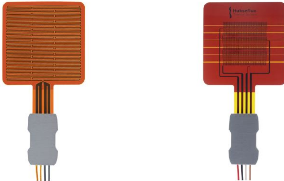
Figure 0.1 On the left HTR01 heater for calibration and verification of performance of FHF-type heat flux sensors, on the right an FHF01 heat flux sensor to which HTR01 may be applied. See also figure 3.2.1 for dimensions.
