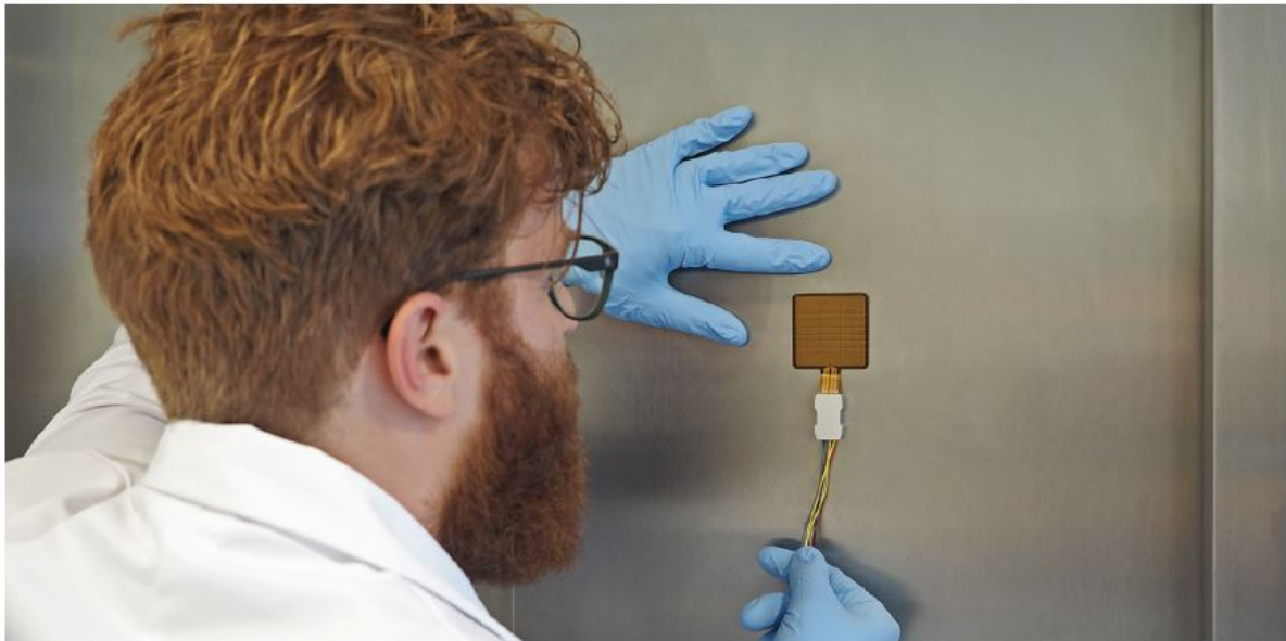
Figure 0.2 Working with HTR01: application of HTR01 on an FHF-type sensor for performance verification. HTR01 is a foil heater. Either it can be used as a general-purpose heater or it can be used in combination with foil heat flux sensors such as FHF01 and FHF02 for test and calibration purposes.
