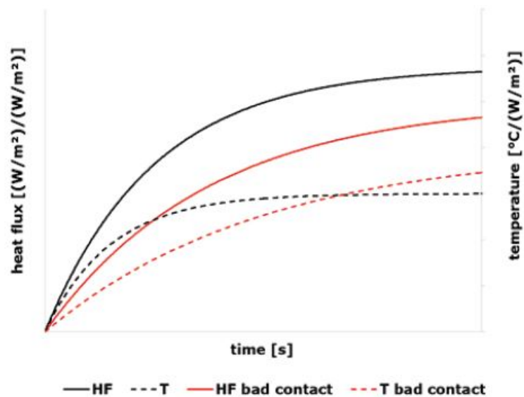
Figure 2.4.1 In situ sensor stability check. Comparison of responses to stepwise heating relative to reference curves. Normalised to heater power (P) and relative to the heat flux and the temperature just before heating. Solid graphs show heat flux, dotted graphs show temperature. The black HF and T signals are the reference curves at good thermal contact. The sensor loses thermal contact, which results in the red responses: slower response times, lower heat flux and higher temperature rise.
