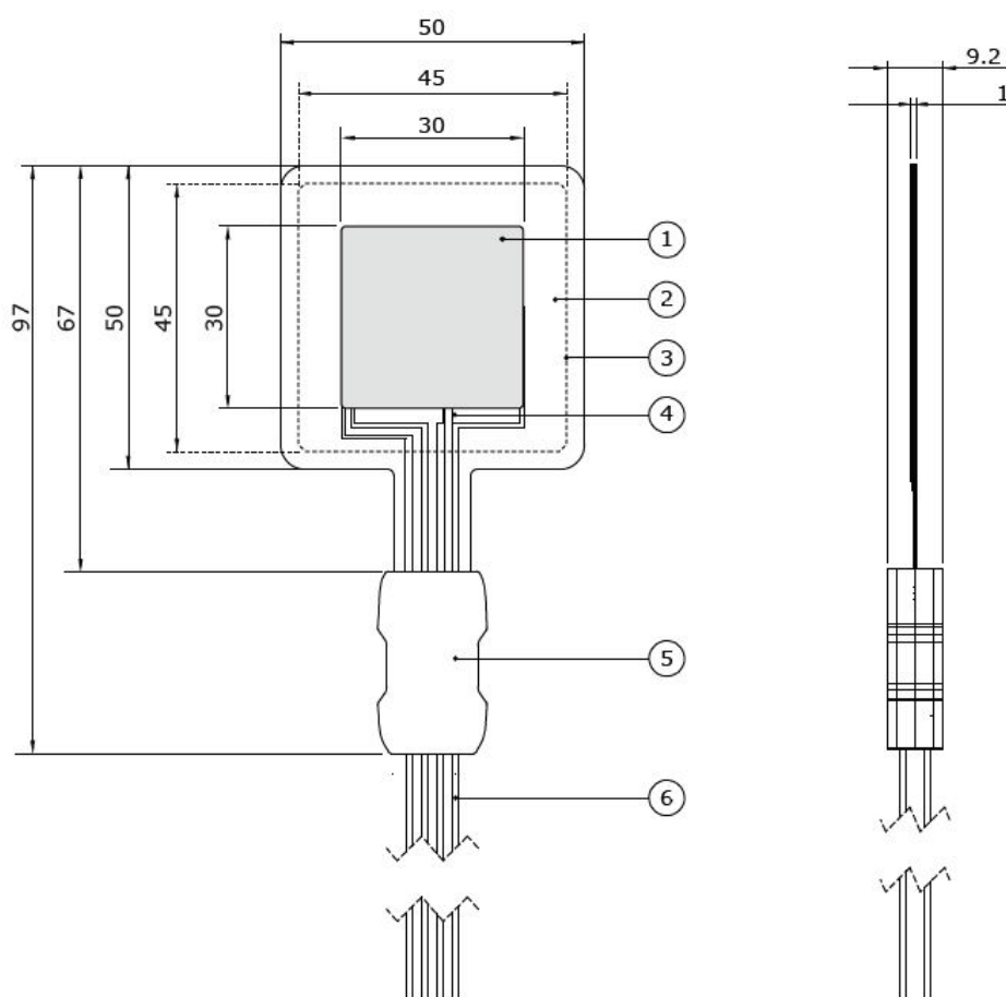
FHF02SC heat flux sensor; dimensions in \times 10^{-3} m
