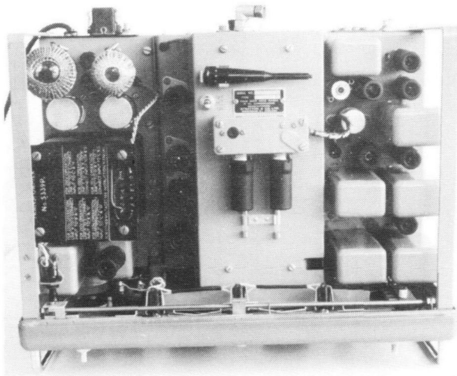
Eddystone 730/4: Above-chassis view with case removed
