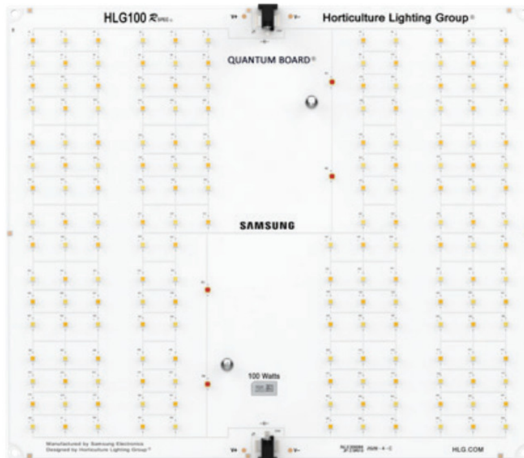
HLG 100 R Spec Lamp
