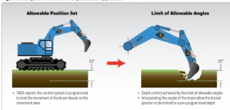
Figure 2. Honeywell TARS-IMU in a Depth Control Application
