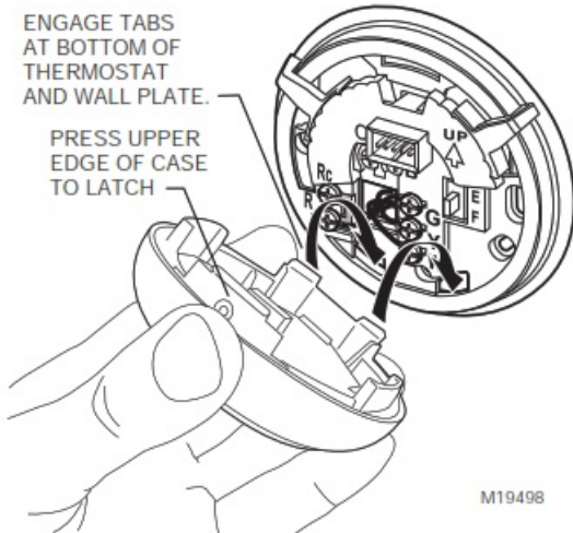
Fig. 9. Mounting thermostat to wallplate.
