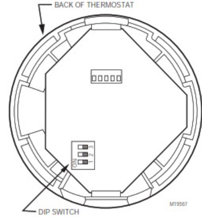
Fig. 8. DIP switch.
