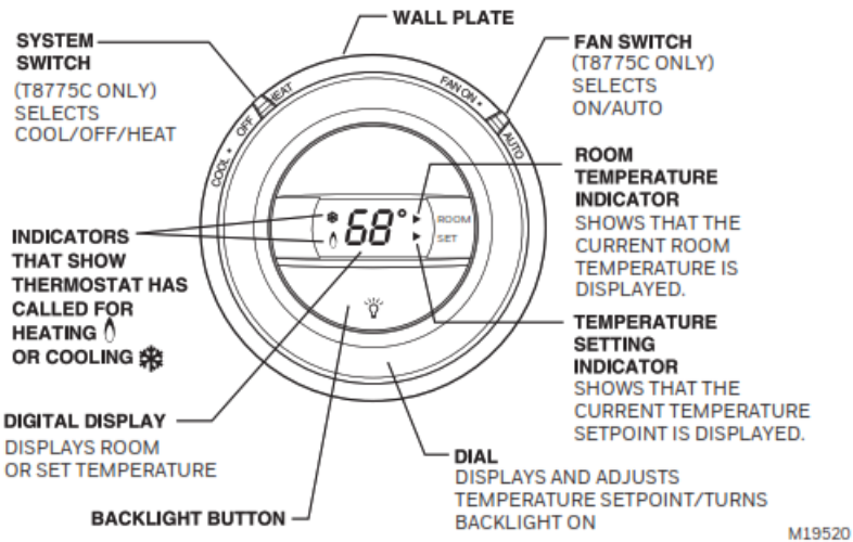
10. Fig. 10. T8775 Thermostat (features and operation).
