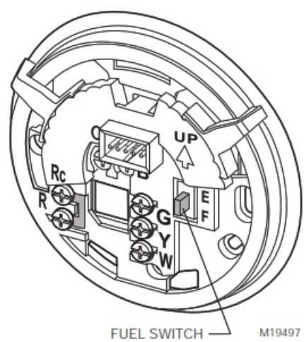
Fig. 7. Fuel switch.
