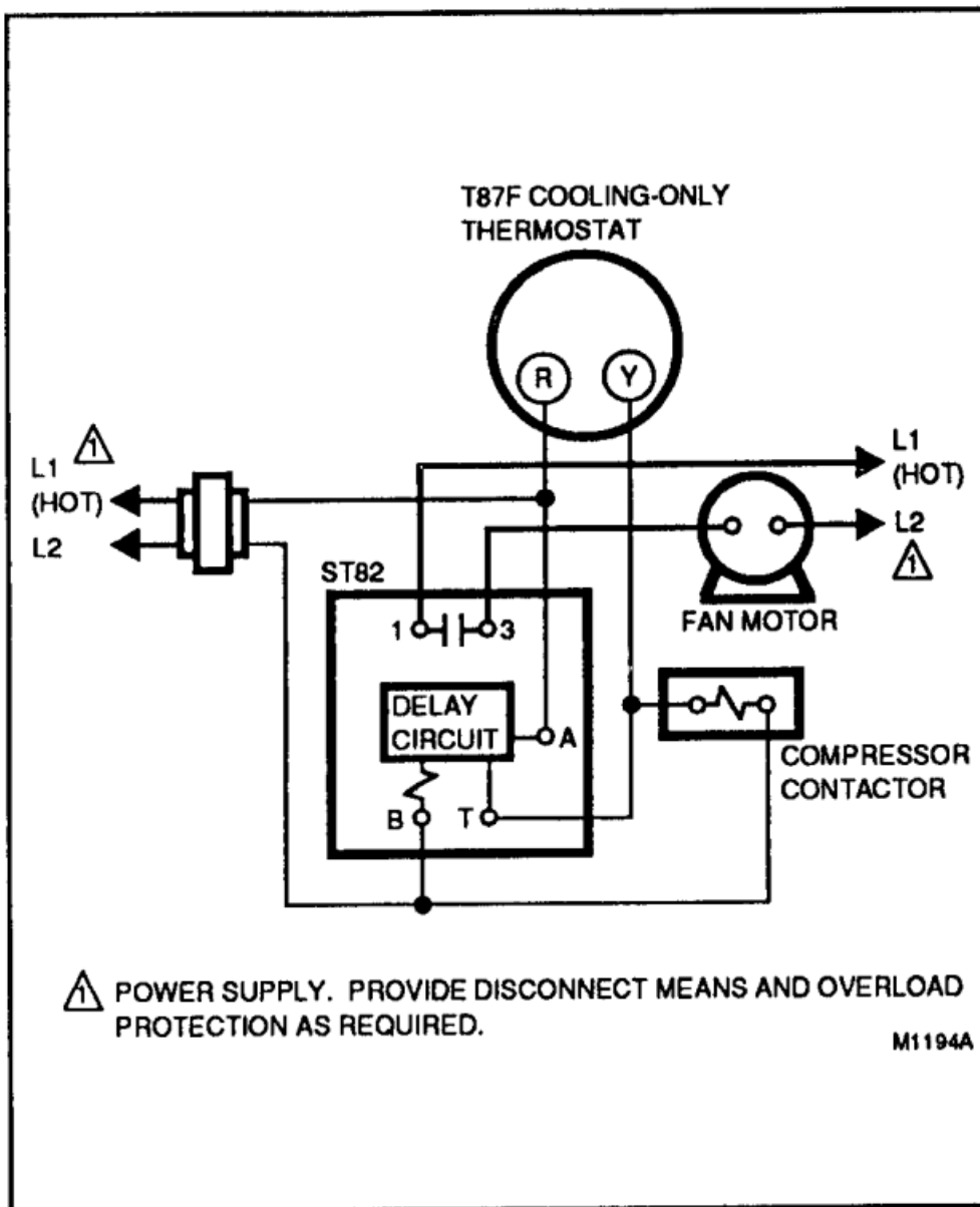
FIG. 6-ST82 IN A HEAT PUMP APPLICATION.
