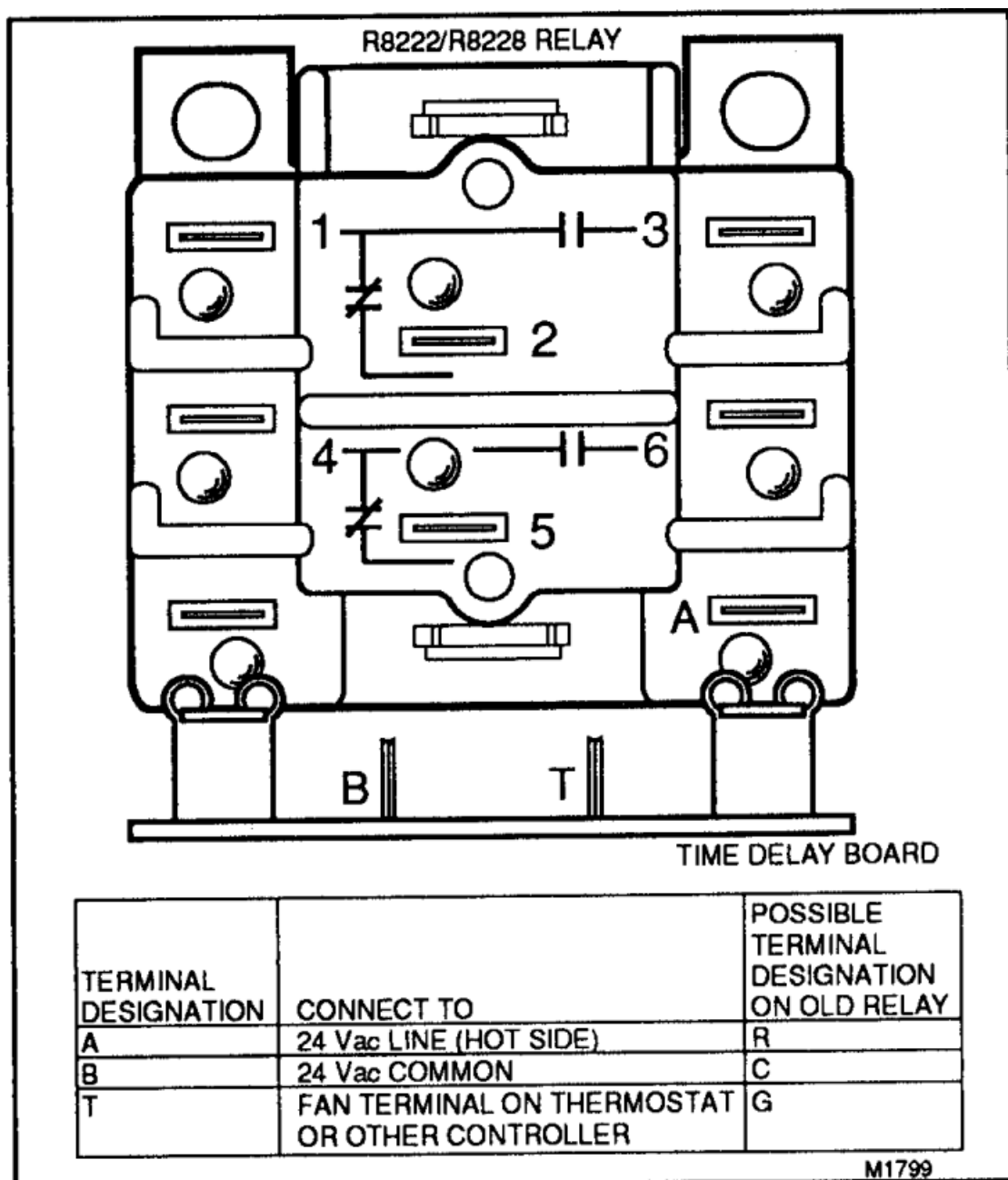
FIG. 5-ST82 IN A COOLING-ONLY APPLICATION.
