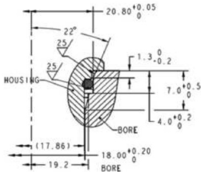
FIGURE 4. CUSTOMER INTERFACE BORE
