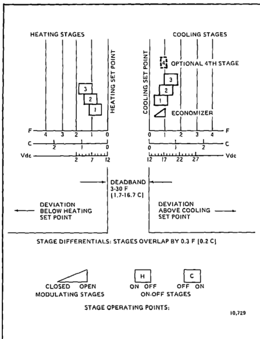
FIG. 1-W7080A STAGE OPERATING POINTS, DIFFERENTIALS, AND THROTTLING RANGES.
