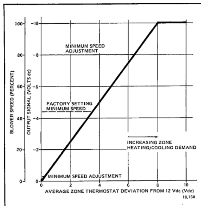
FIG. 6-HOT DECK LIMIT- MINIMUM VOLTAGE OUTPUT.
