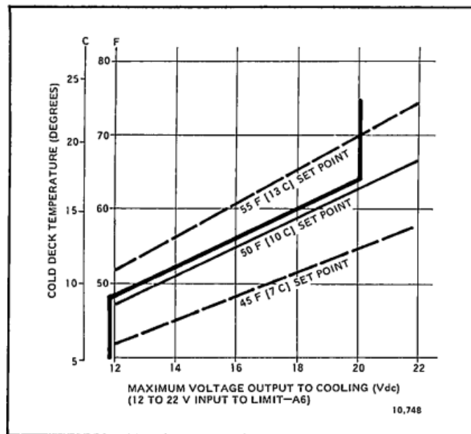
FIG. 4-ECONOMIZER/MIXED AIR LOW LIMIT-MAXIMUM VOLTAGE OUTPUT.
