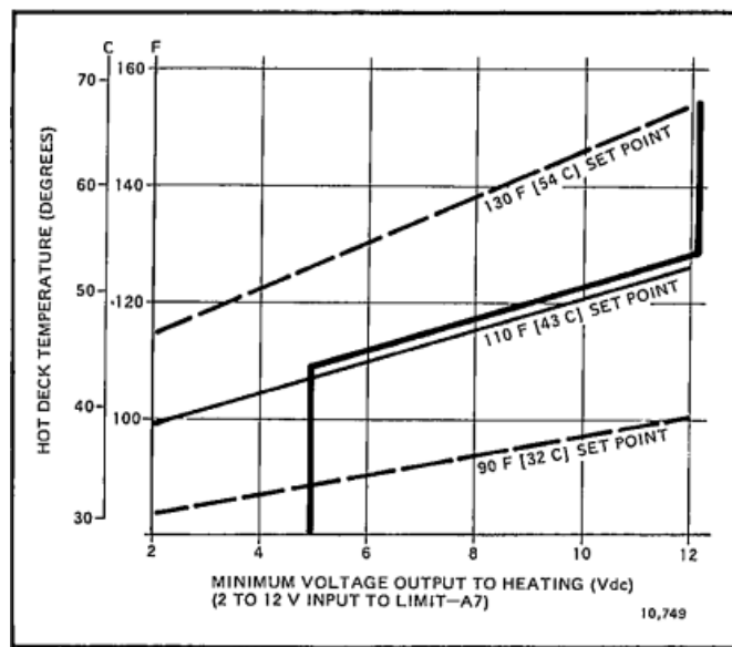
FIG. 5-COLD DECK LOW LIMIT-MAXIMUM VOLTAGE OUTPUT.
