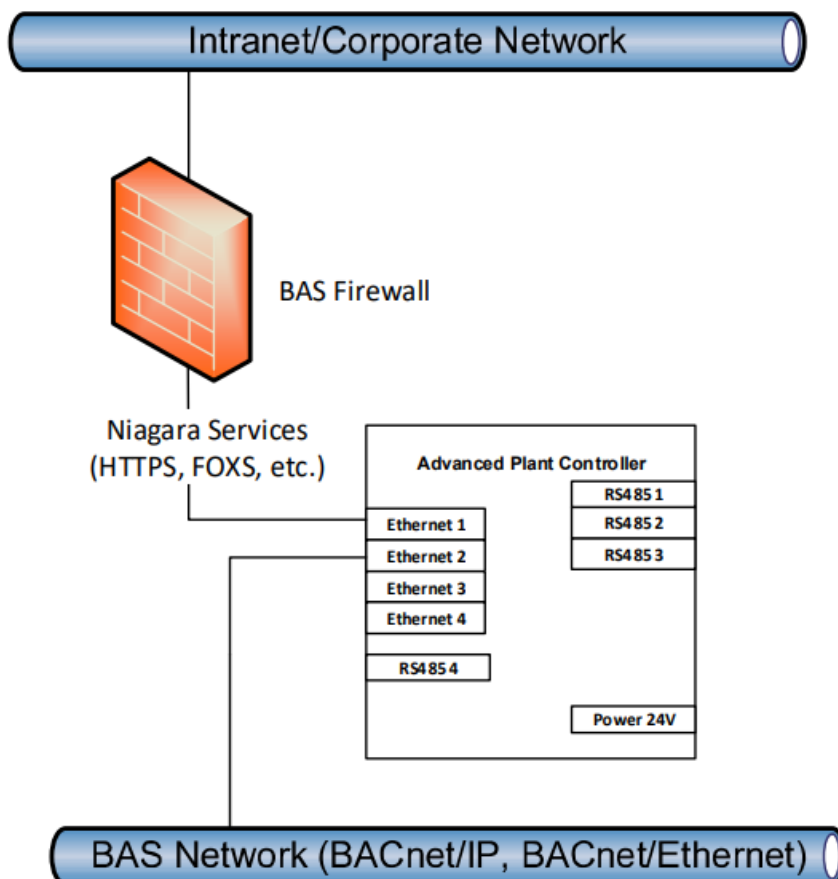
Fig. 3 BACnet™ and Niagara Connections
