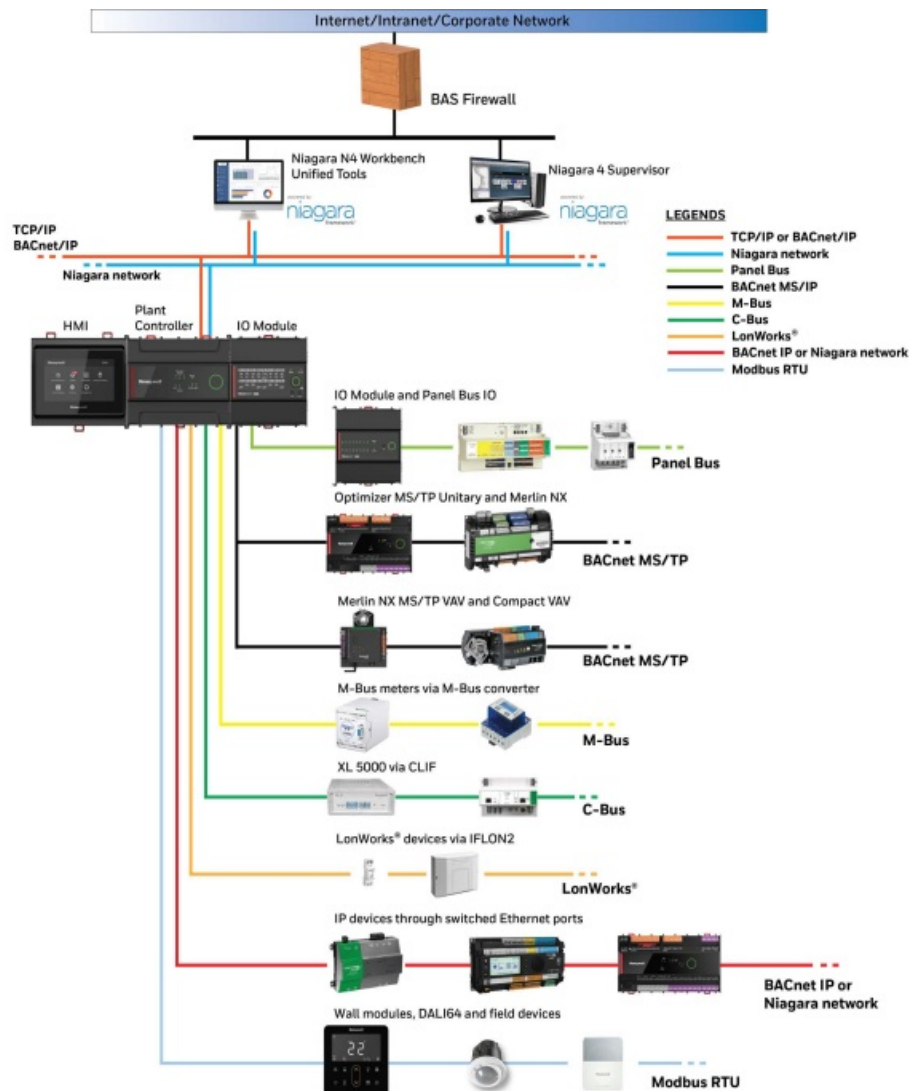
Fig. 1 System Overview
