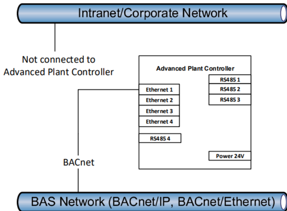
Fig. 2 BACnet™ Connection
