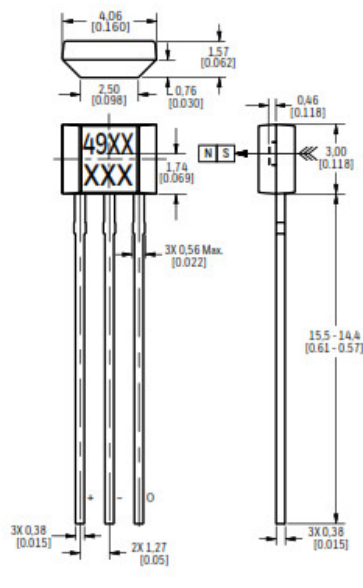
Figure 4. SS490 Series Flat TO-92-Style Mounting and Dimensional Drawings (For reference only: mm/[in.] )
