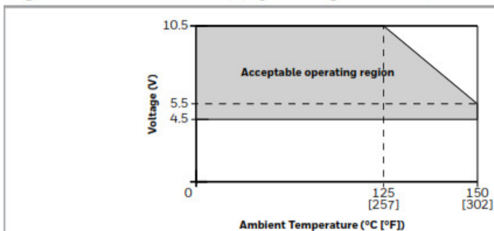
Figure 2. Maximum Supply Voltage vs Temperature
