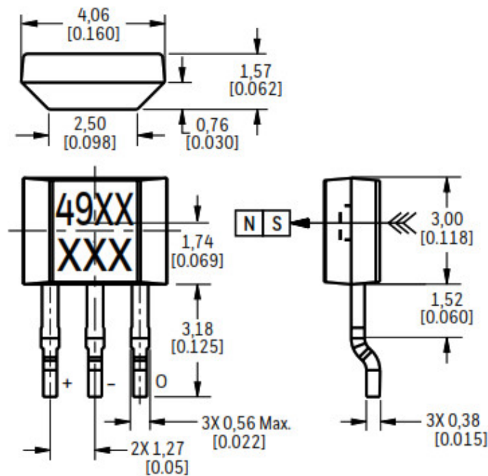
Figure 4. SS490 Series Flat TO-92-Style Mounting and Dimensional Drawings (continued) E. Surface Mount Sensor IC, Bulk Pack
