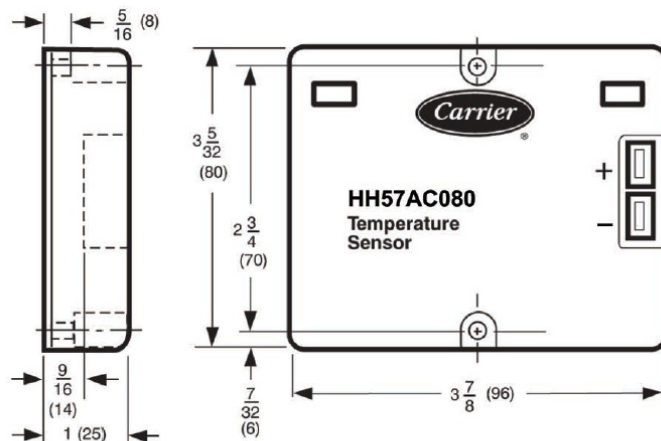
Fig. 4 — Temperature Sensor Specifications
