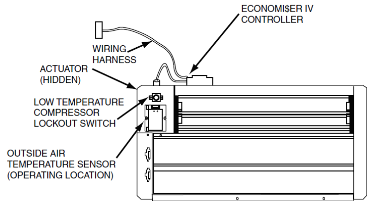
Fig. 2 — EconoMi$er IV Component Locations
