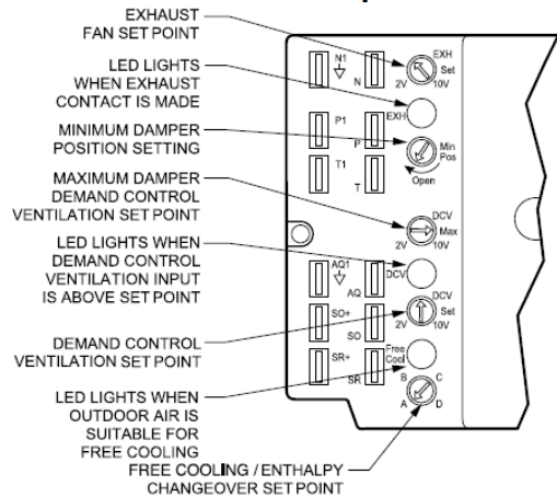
Fig. 3 — EconoMi$er IV Controller Potentiometer and LED Locations
