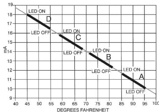
Fig. 5 — Outdoor Air Changeover Temperature
