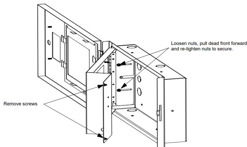
Figure 2 ECS-RPU Dead Front Open 180°
