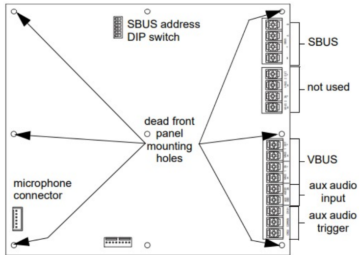
Figure 3 Back View of ECS-RPU
