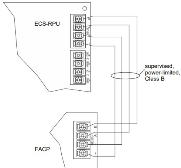
Figure 4 Wiring the ECS-RPU to the FACP
