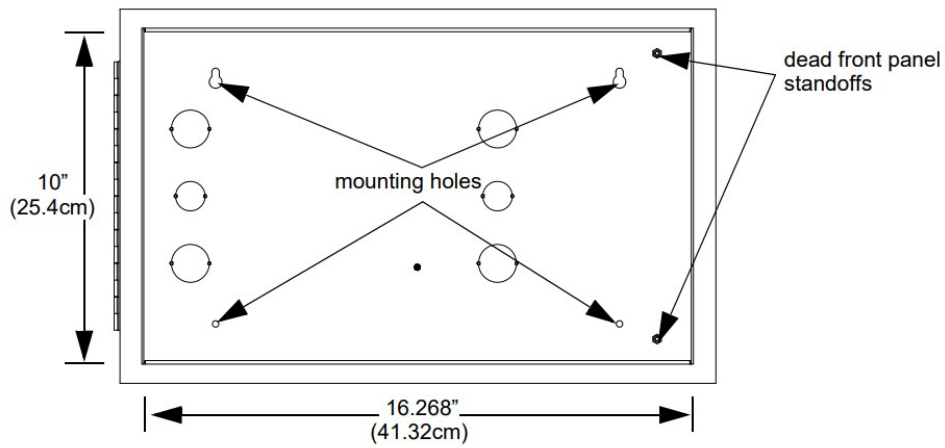
Figure 1 Cabinet Mounting Holes
