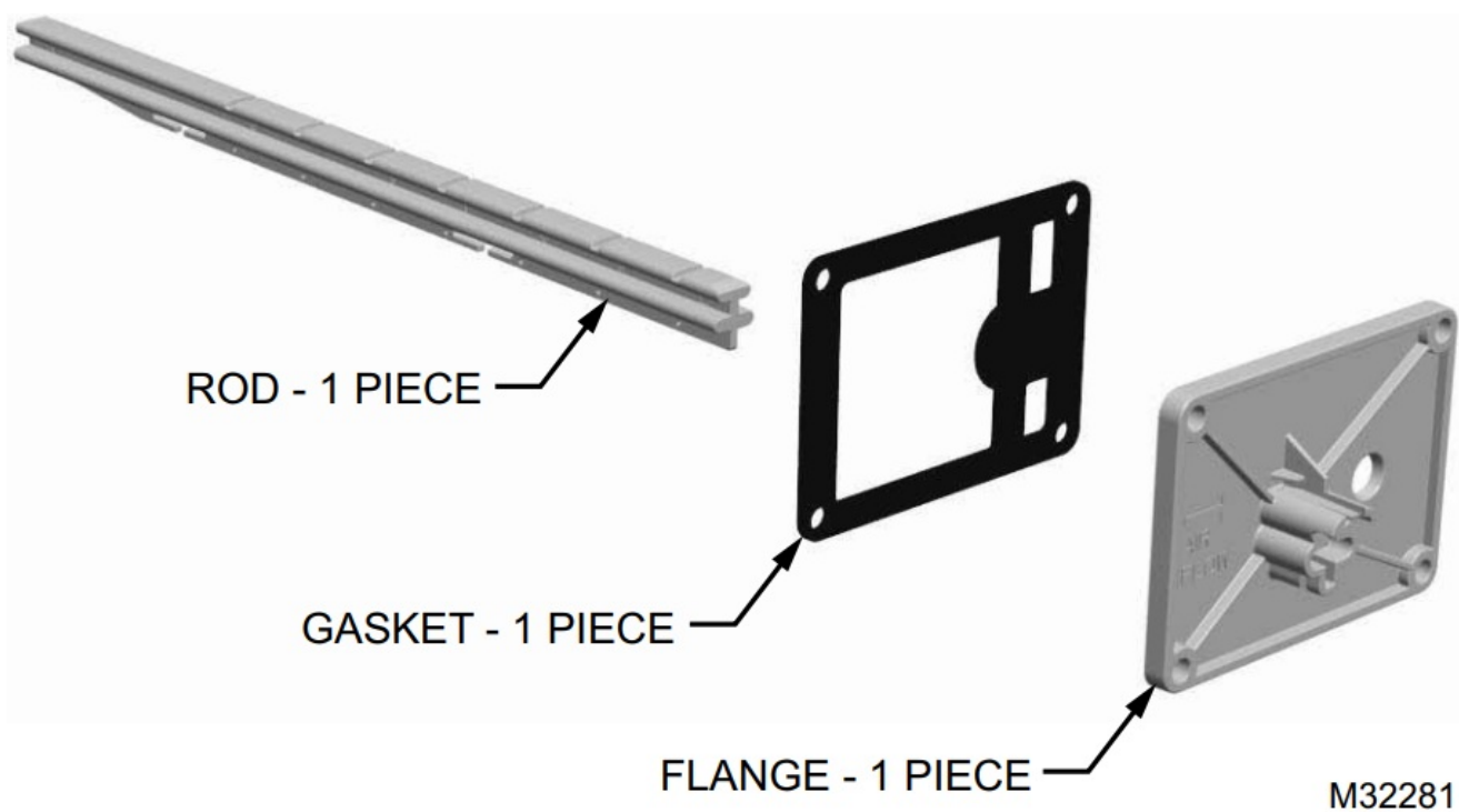
Fig. 2. Duct Mounting Kit (Part # 50053060-001).
