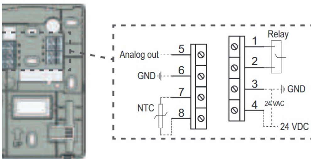
Figure 3. Typical wiring connections
