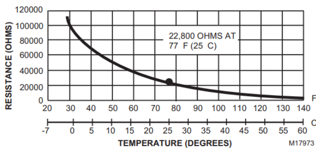
Fig. 8. C7046B Sensor resistance vs. temperature.
