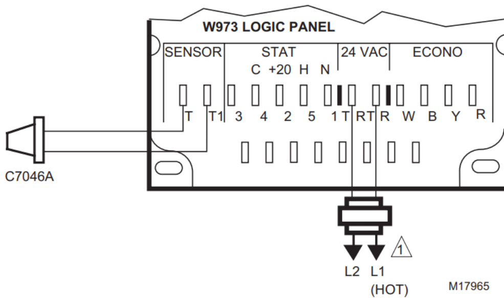
Fig. 4. Connecting C7046A Air Temperature Sensor to a W973 Single Zone Logic Panel.
