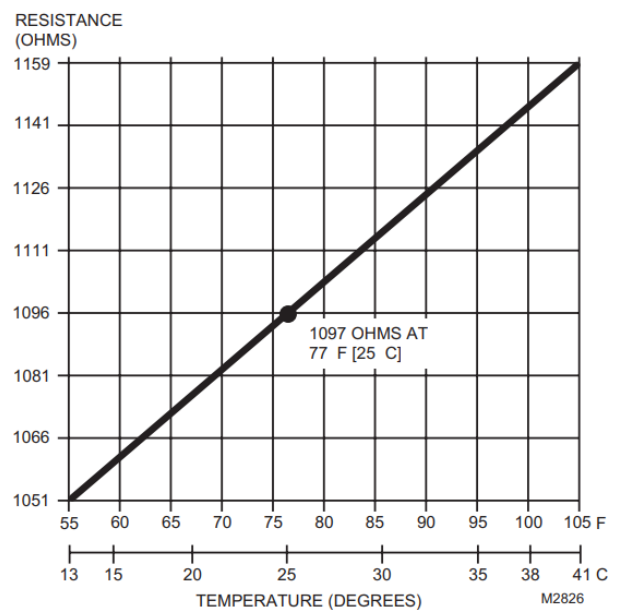
Fig. 9. C7046D Sensor resistance vs. temperature.
