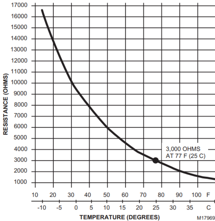
Fig. 7. C7046A,C Sensor resistance vs. temperature.
