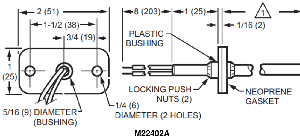
Fig. 1. C7046A,B,C,D Air Temperature Sensor dimensions in in. (mm).
