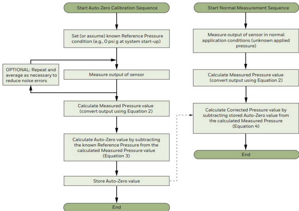
Figure 4. How to Implement Auto-Zero Calibration and Correction
