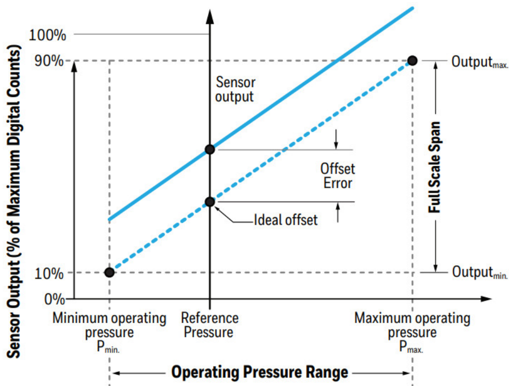
Figure 3. Transfer Function of Digital Sensor with Offset Error (10% to 90% Calibration)
