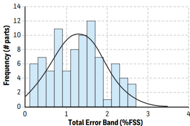
C. Total Error Band over Operating Temperature (0°C to 50°C) and Operating Pressure Range
