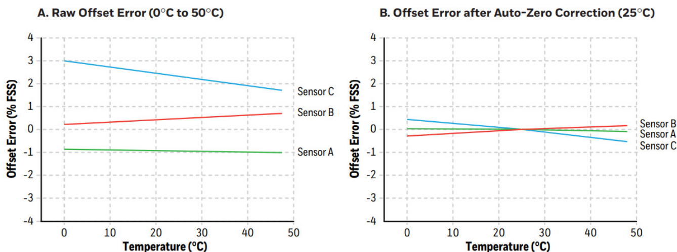
Figure 5. Auto-Zero Calibration Example
