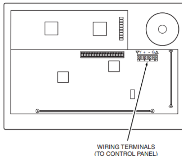
Figure 2 - 6160RF Wiring Details
