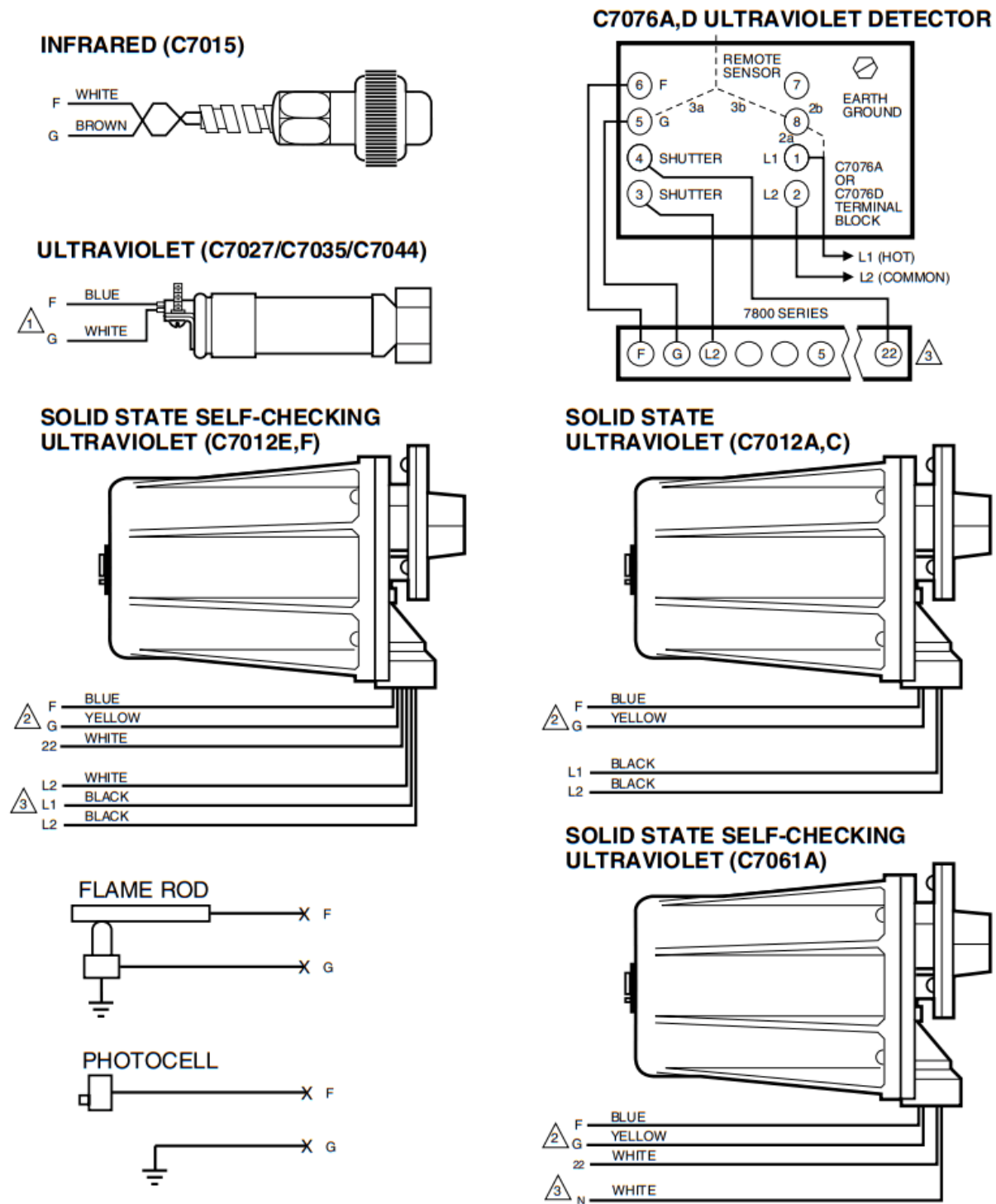
Fig. 14. Flame detector wiring.
