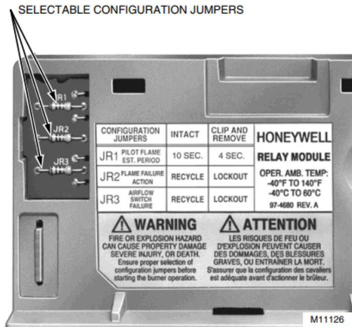
Fig. 17. Selectable site-configurable jumpers.
