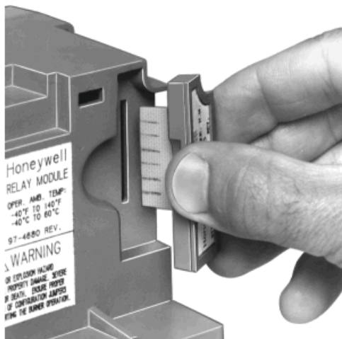
Fig. 11. ST7800 Purge Card installation.
