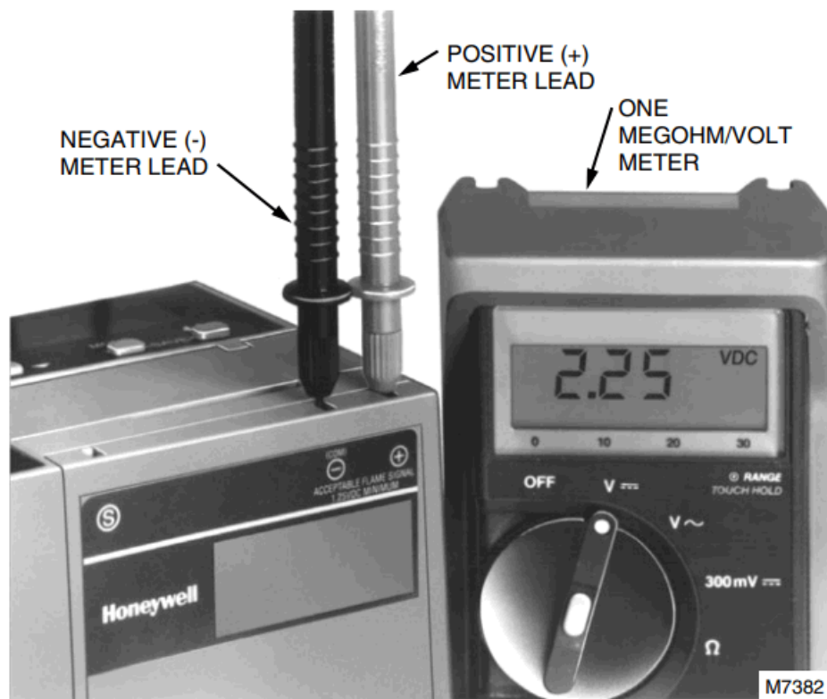
Fig. 18. Flame signal measurement.
