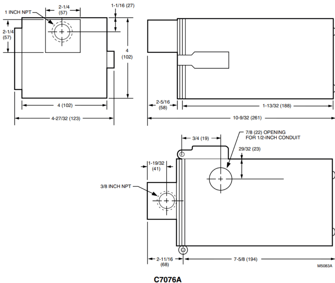
Fig. 4. Ultraviolet detectors in in. (mm).
