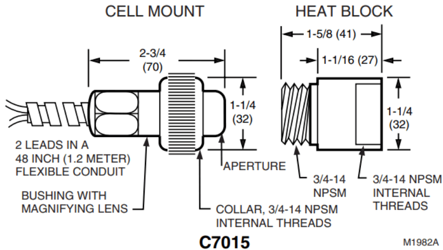
Fig. 5. Infrared detector in in. (mm).
