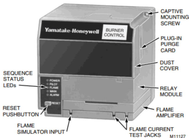
Fig. 16. Sequence status LEDs.
