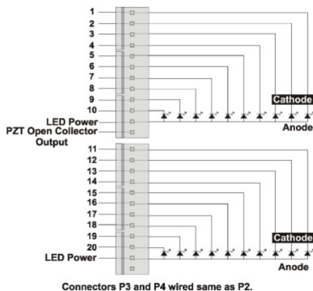
LED Wiring
