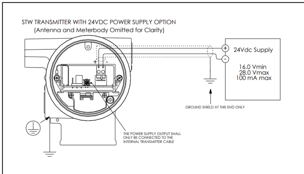
Figure 5: Power Supply 24Vdc Option (DC) System Diagram
