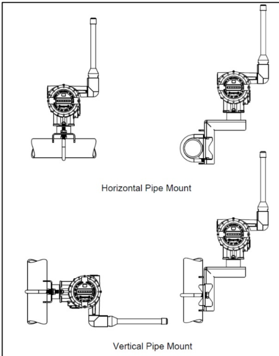
Figure 2: Mounting Brackets
