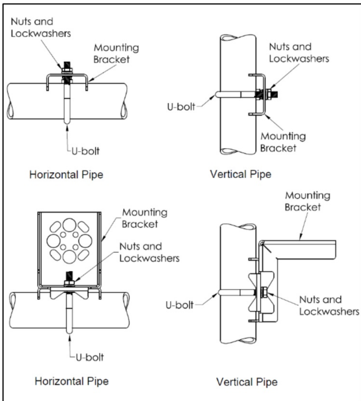
Figure 1: Flat and Angle Mounting Brackets
