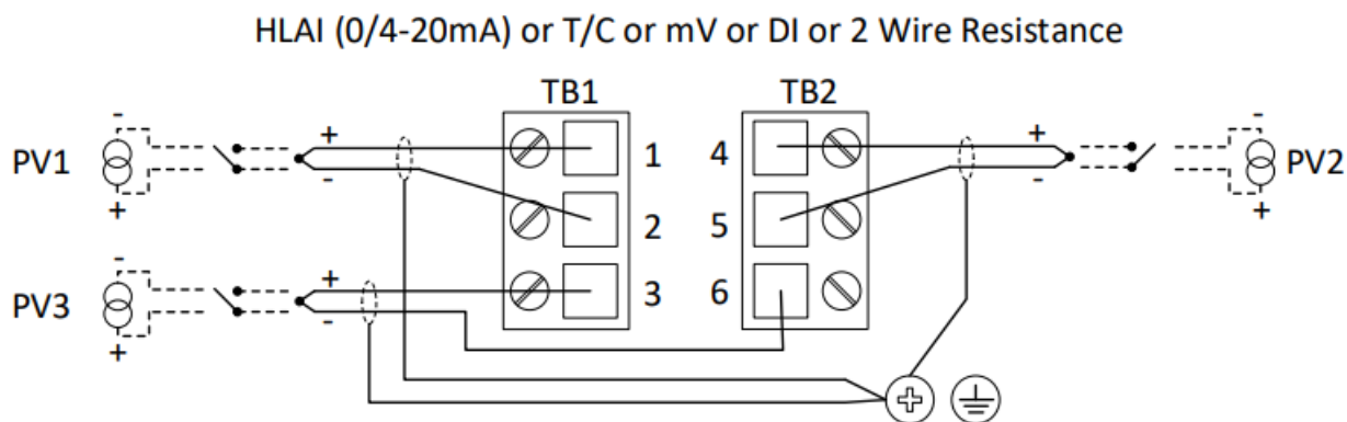
Figure 7: STUW750 Universal I/O Transmitter Connections
