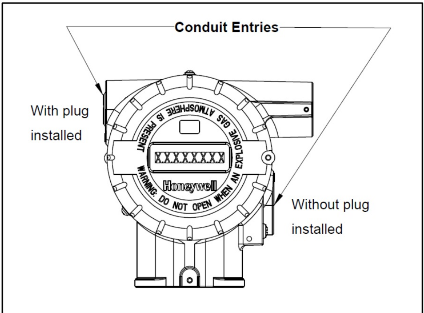
Figure 4: Electronic Housing Conduit Entries
