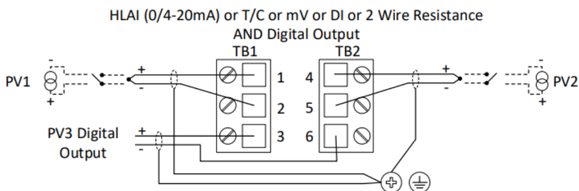
Figure 8: STUW751 Universal I/O Transmitter Connections
