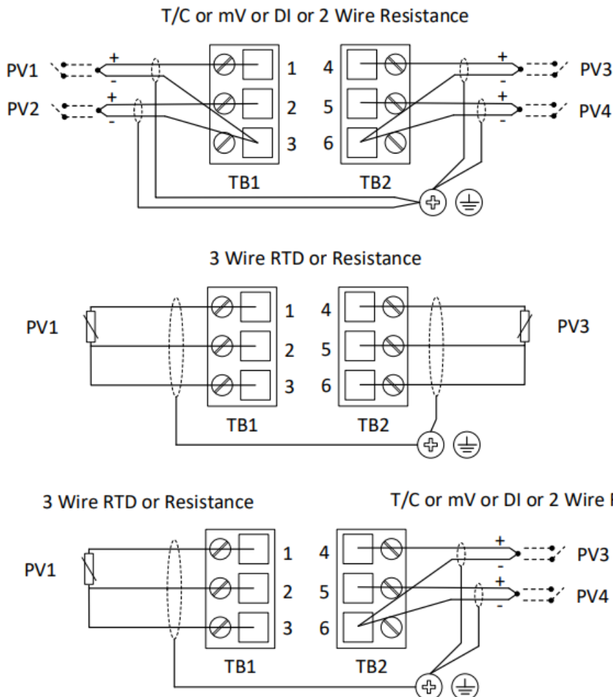
Figure 6: STIW400 Temperature Transmitter Connections
