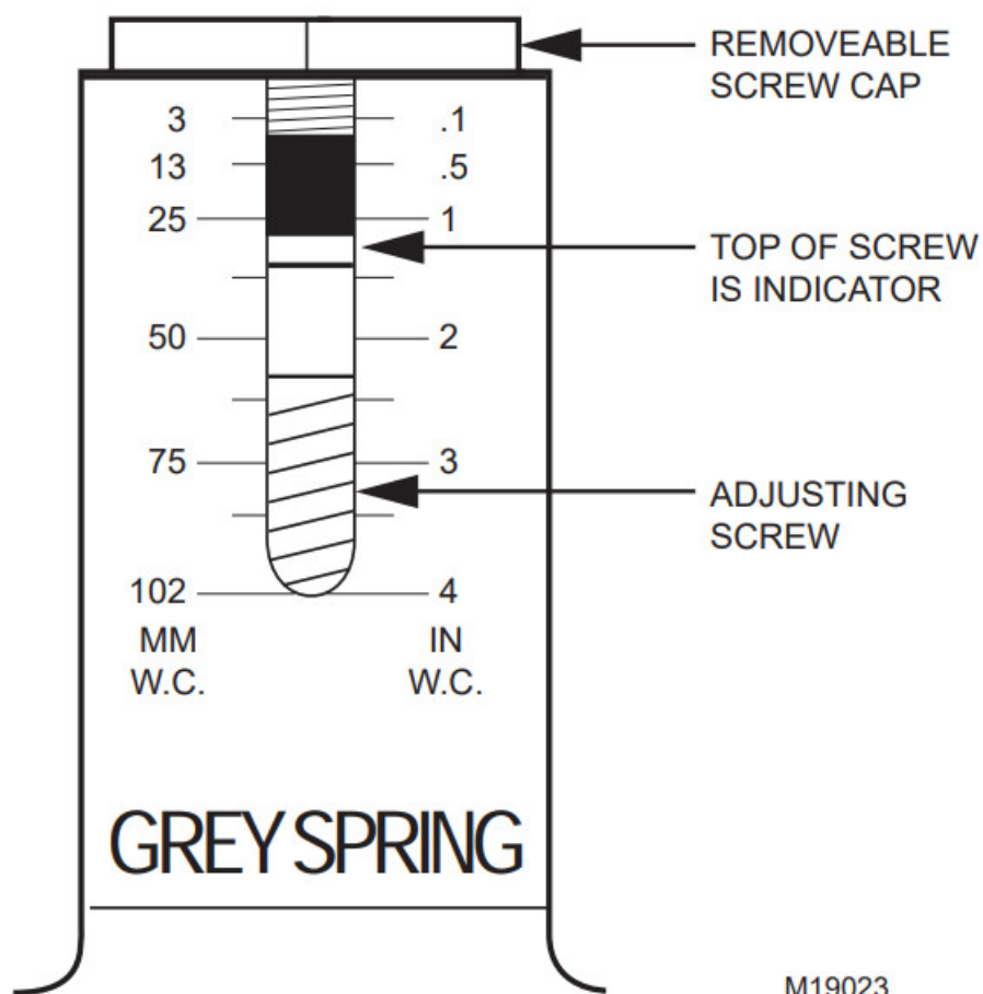
Fig. 6. Static pressure range settings.
