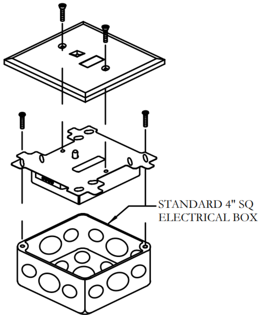
FIGURE 2 TYPICAL MOUNTING ARRANGEMENT
