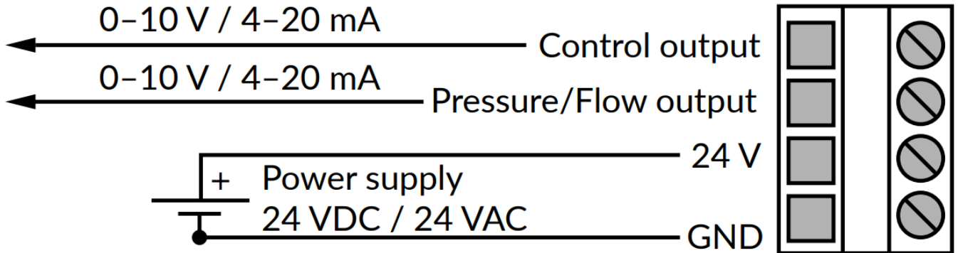
Figure 2b – Output mode selection: Default selection 010 V for both
