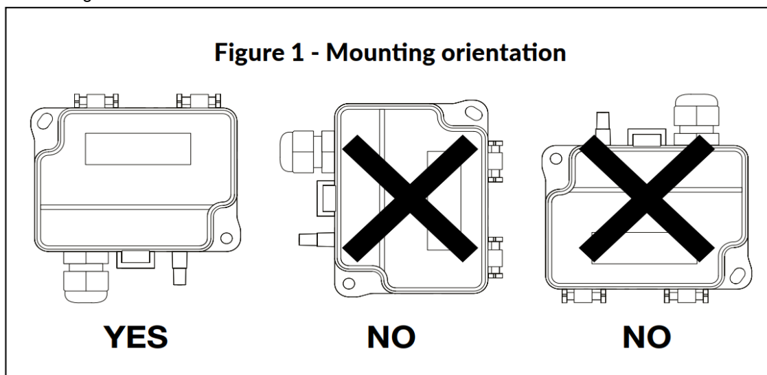
Figure 1 – Mounting orientation
