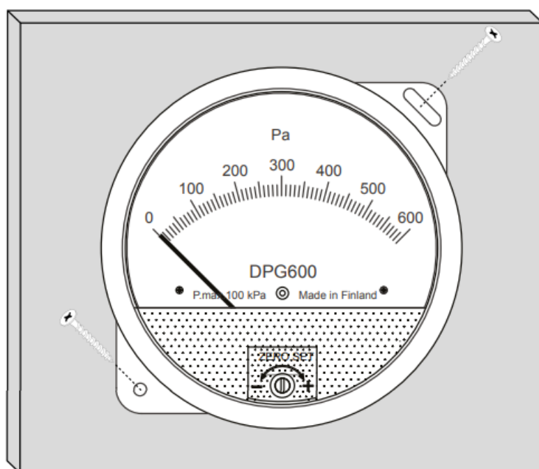
Surface mount
