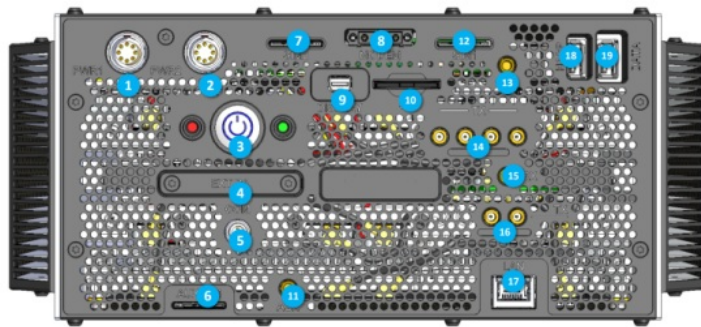
Figure 3: System Top Panel
