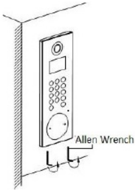
Figure 3-5 Tighten the Screws of Device
