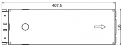
Figure 3-6 Front View
