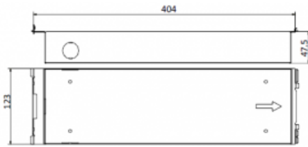
Figure 3-1 Front and Side View
