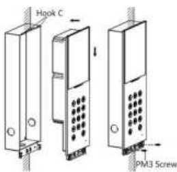
Figure 3-10 Install the Door Station
