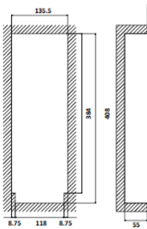
Figure 3-8 Dimensions of the Hole
