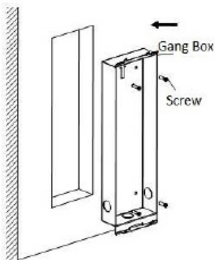
Figure 3-3 Insert the Gang Box into the Wall
