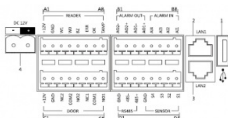
Figure 2-2 Terminals and Interfaces of DS-KD6002-VM
