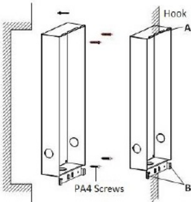
Figure 3-9 Insert the Gang Box into the Wall
