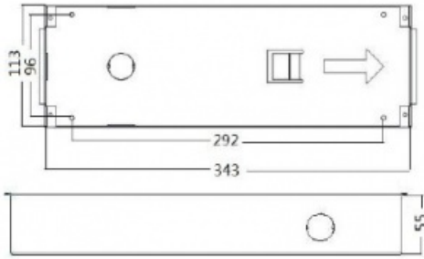
Figure 3-12 Front and Side View
