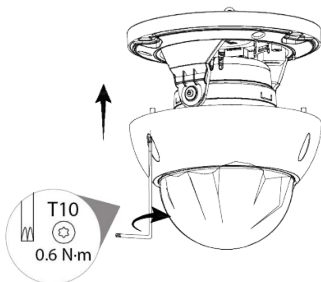
Figure 3-11 Close the Camera
