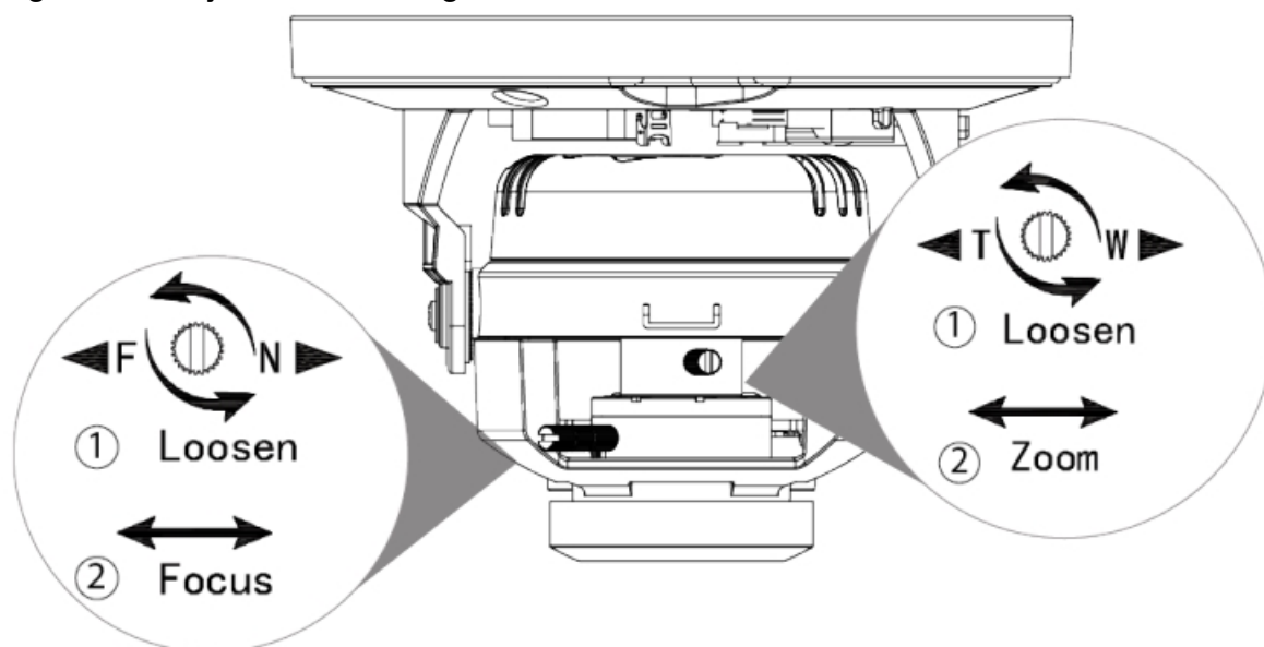
Figure 3-12 Adjust the focal length
