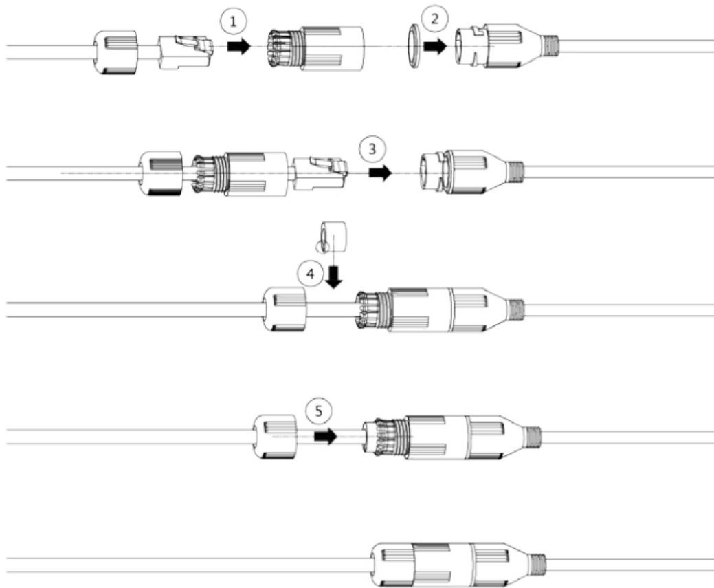
Figure 3-9 Install the waterproof connector
