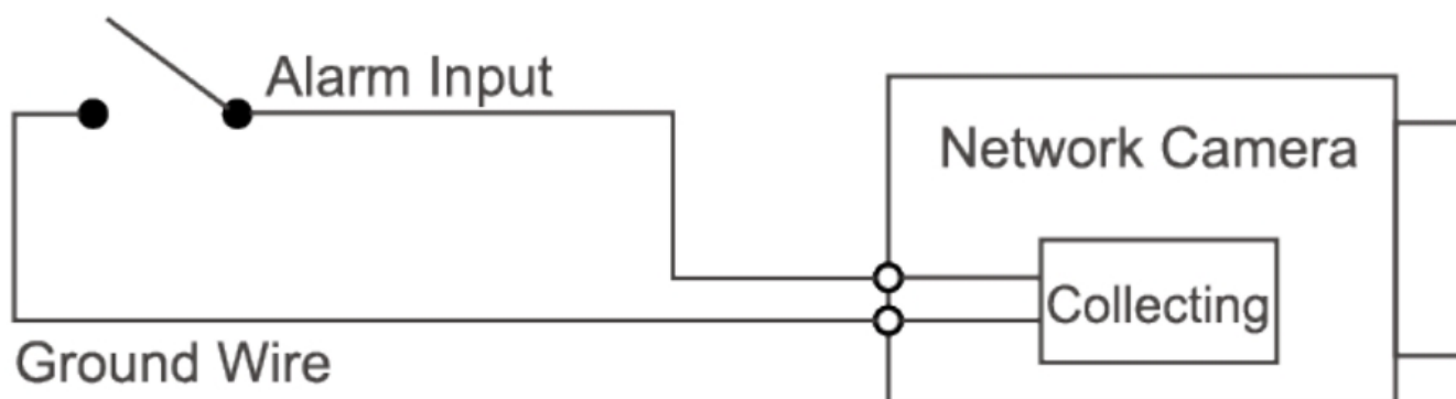
Figure 1-2 Alarm input
