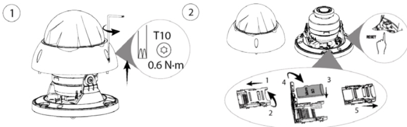
Figure 3-6 Install the SD card
