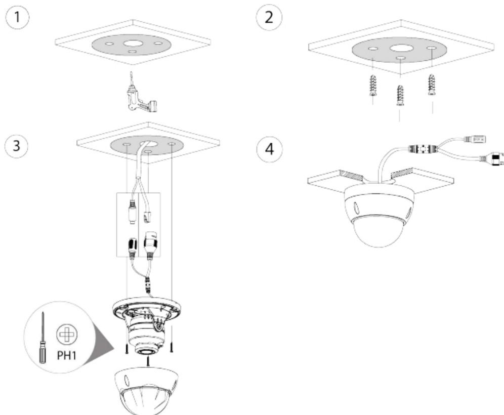
Figure 3-8 Cable going through the mounting surface
