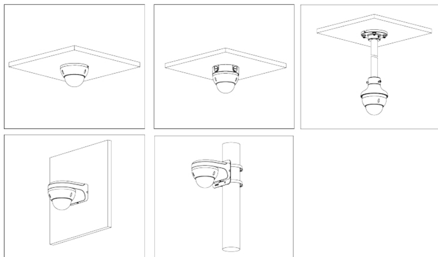
Figure 3-5 Installation methods
