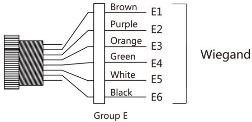
Figure 2-2 Wiegand Interface Description
