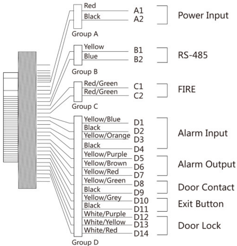
Figure 2-1 Cable Interface Description Table 2-1 Cable Interface Description
