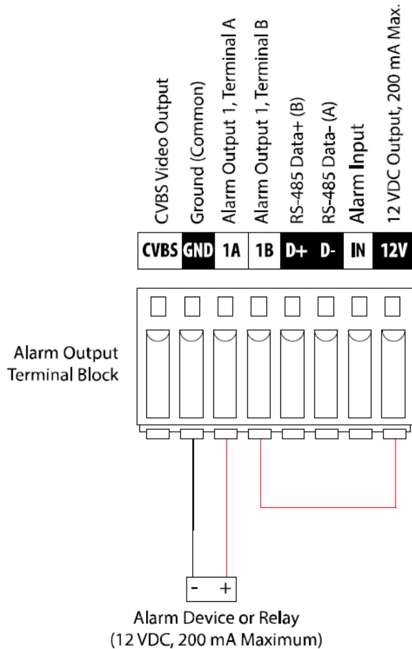
Alarm Output with Power from Camera
