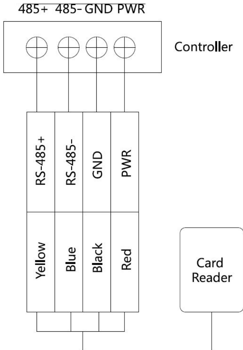
Figure 2-3 Wiring for RS-485 Communication Mode
