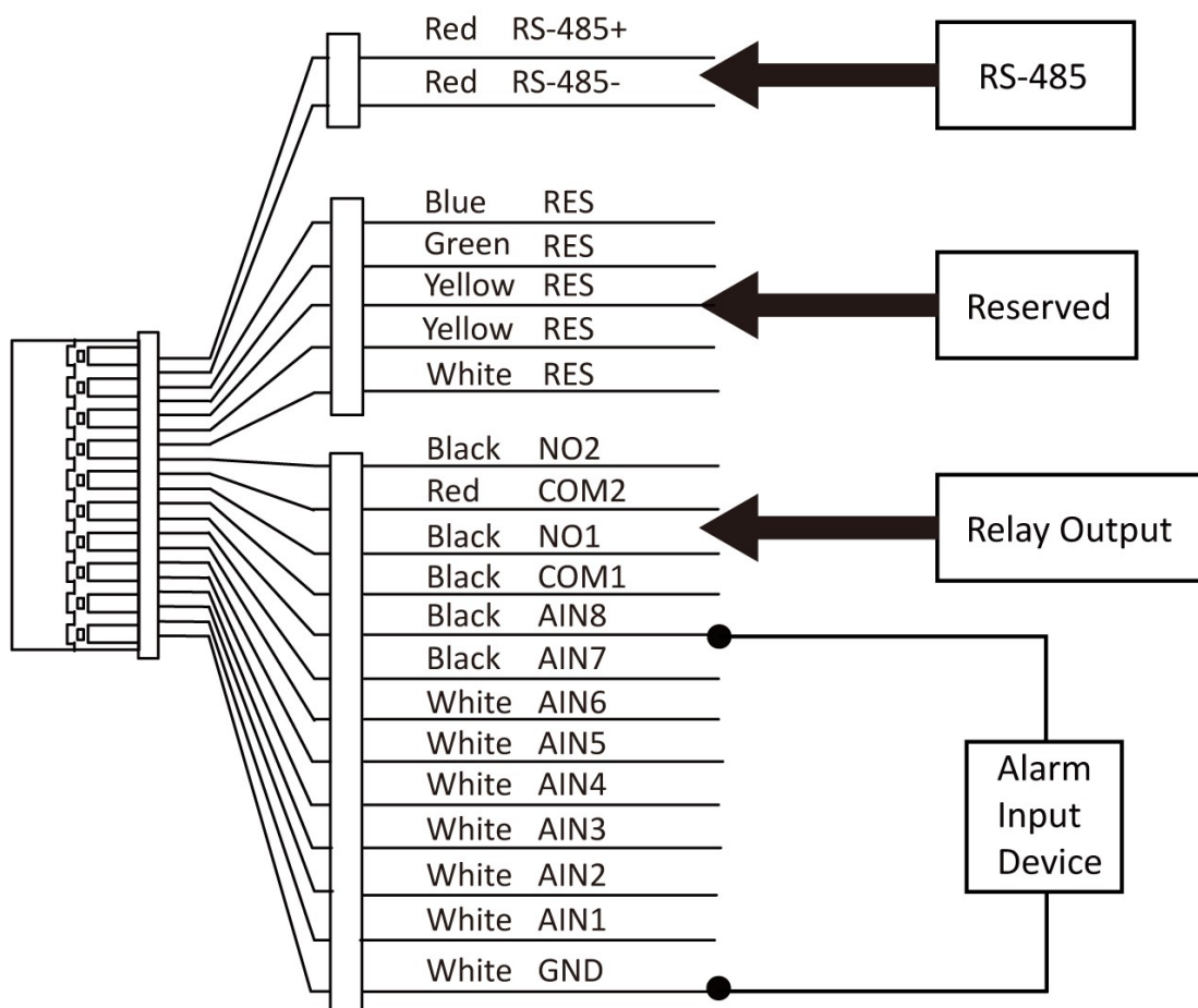
Figure 3-1 Wiring Description (Alarm Input Device)
