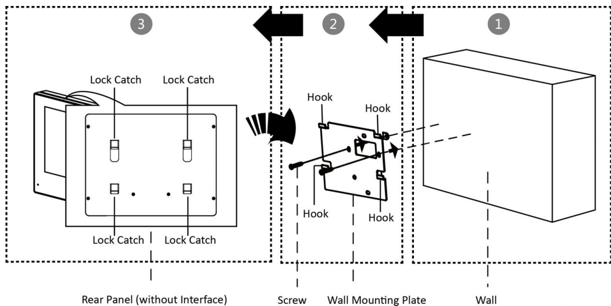
Figure 4-3 Wall Mounting without Junction Box
