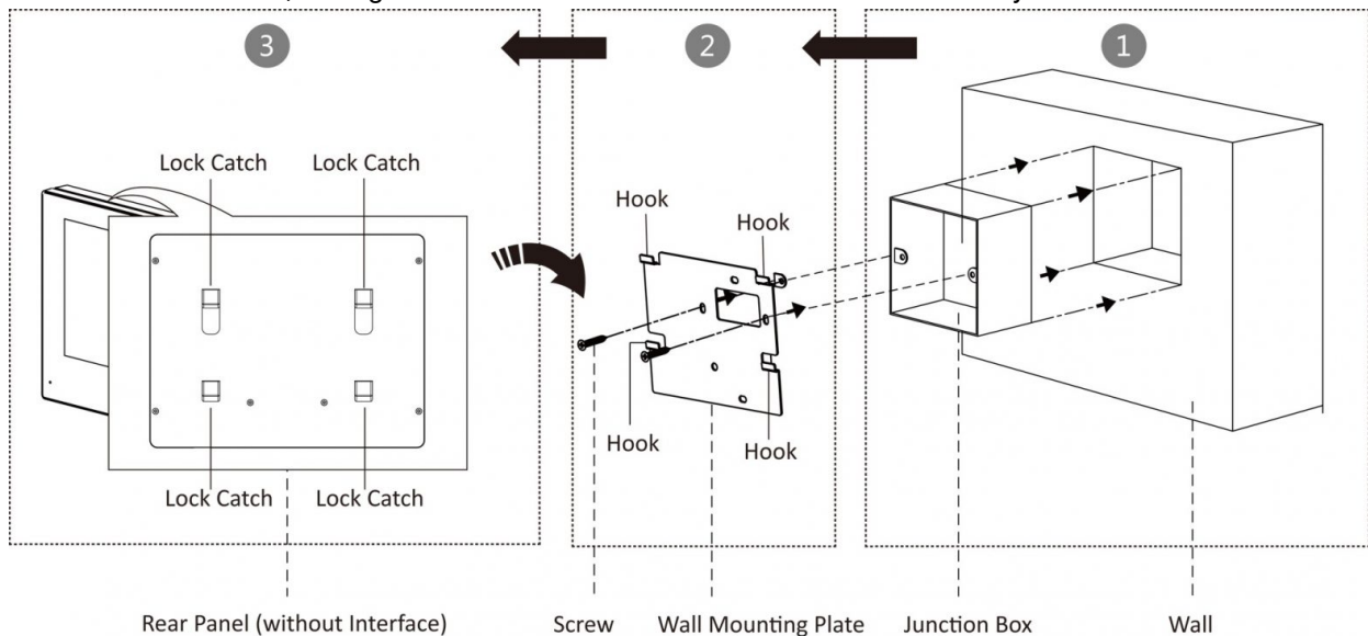
Figure 4-2 Wall Mounting with Junction Box
