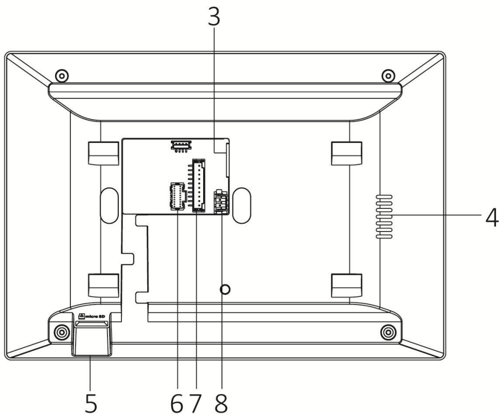
Figure 2-2 Rear Panel Table 2-2 Description
