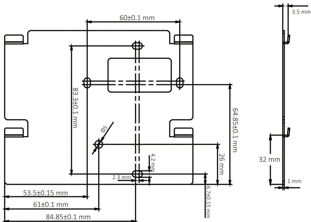
Figure 4-1 Wall Mounting Plate
